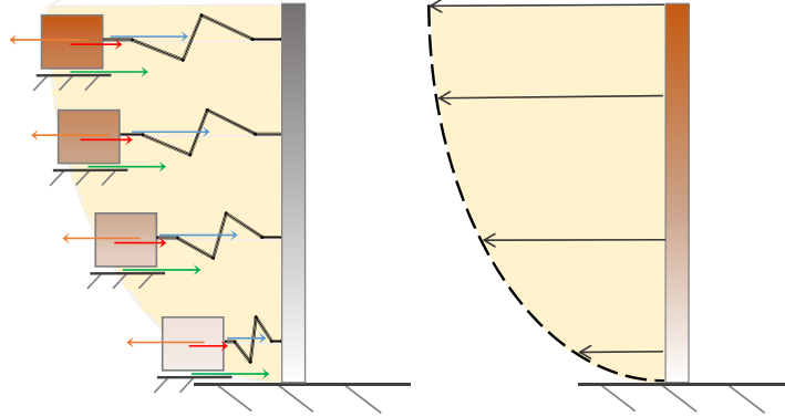
Figure 3: Graphical depiction of the argument: the right-hand side represents the deformation of the stratum as a shear-beam, whereas the left-hand side represents it as a continuous distributions of 1D resonators, where the forces in eq. (11) and fig. 2 are shown in each mass point.
