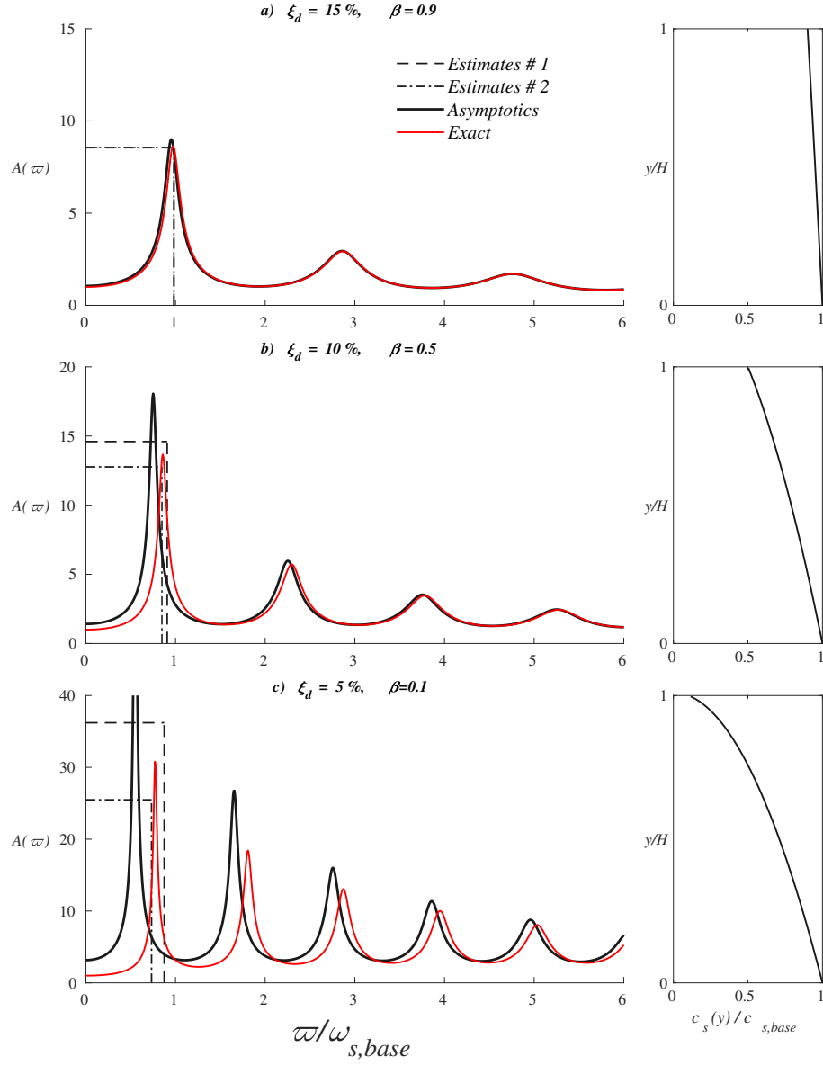
Figure 7: Base-to-top dynamic amplification A(\varpi) (with corresponding vertical S-wave profile c_s(y) ), comparison between eq. (22) with eq. (4) ( Estimates #1 ), eq. (19) with eq. (20b) ( Estimates #2 ), eq. (7) ( Exact ), and eq. (8) ( Asymptotics ) for inhomogeneity factor n = 0.5 and different damping values.
