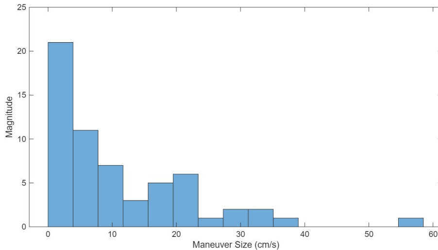
Figure 14: Cislunar station-keeping maneuver size distribution
