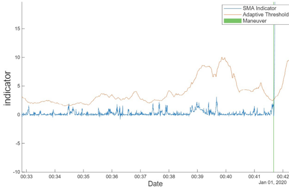
Figure 3: Indicator function from simulated data
