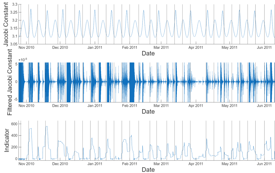
Figure 15: Artemis P2 station-keeping maneuvers
