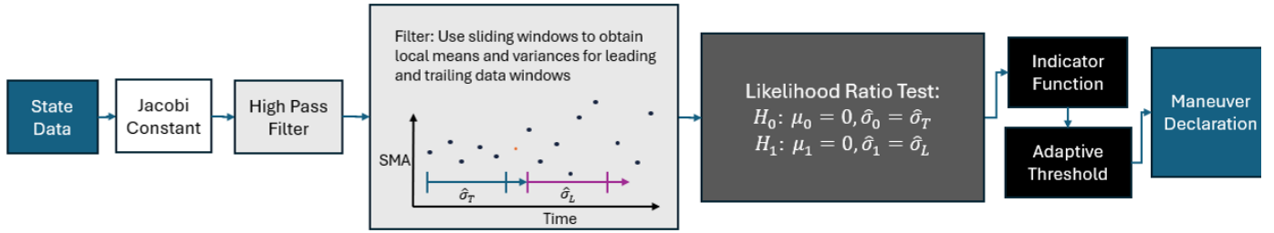
Figure 12: Cislunar algorithm process overview
