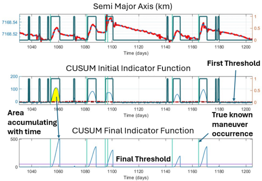
Figure 9: Algorithm execution on data segment
