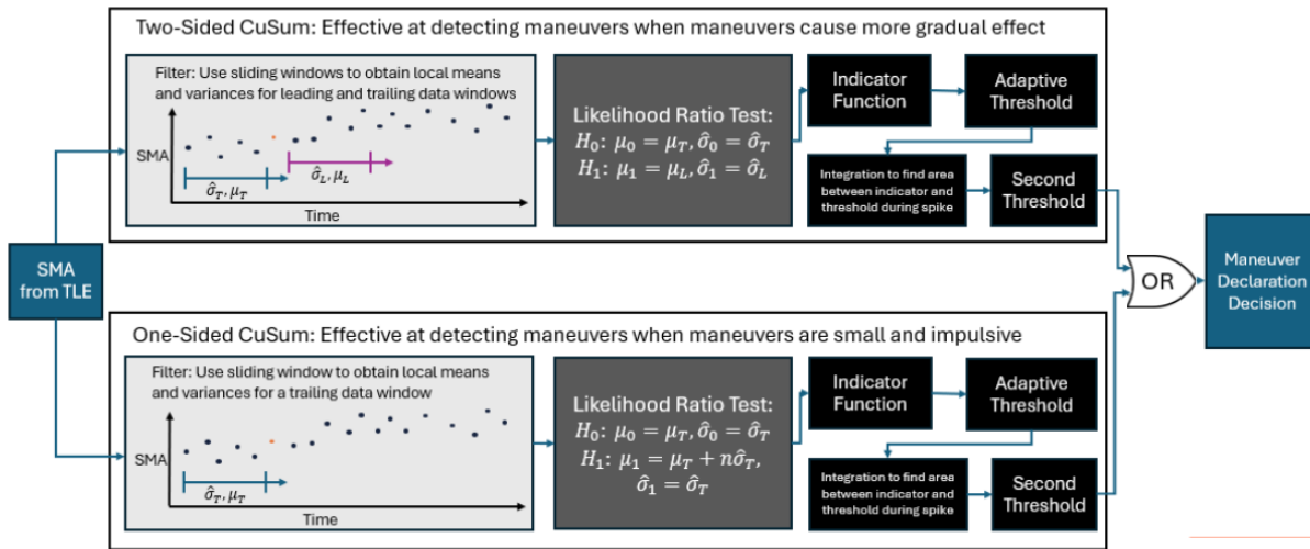
Figure 8: Algorithm process overview
