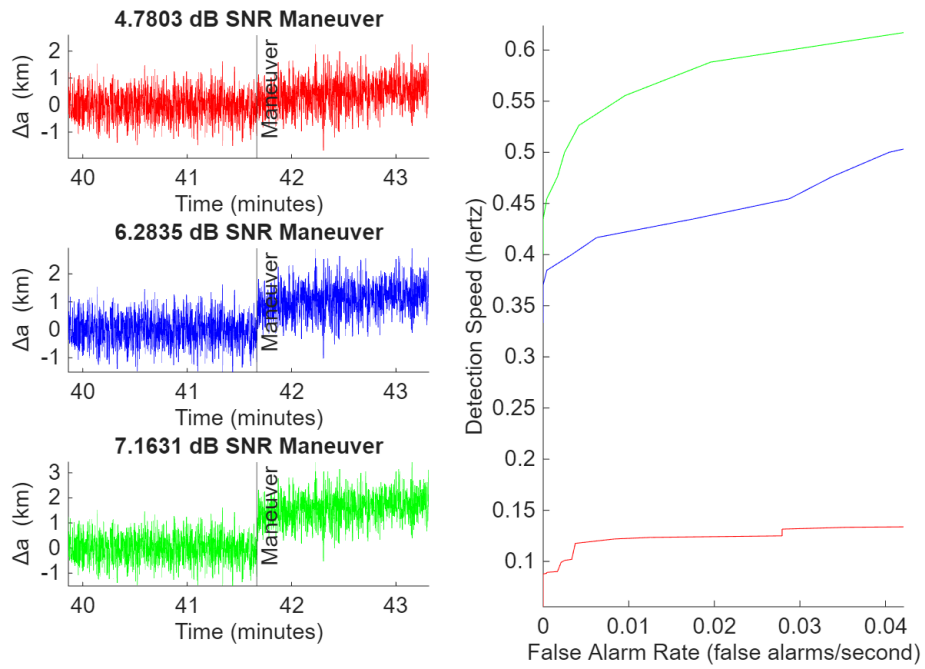
Figure 4: Algorithm results on various magnitude orbit maneuvers in simulation
