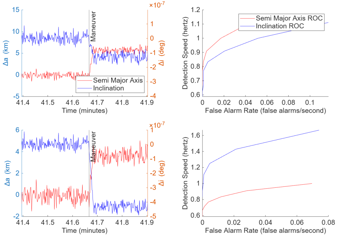
Figure 5: Algorithm results for different monitored invariants under different maneuver directions
