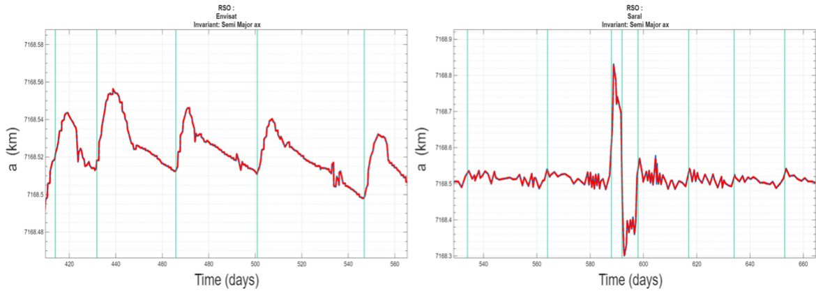
Figure 7: Two segments of TLE data and maneuver times
