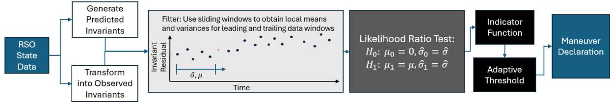
Figure 2: Algorithm overview for maneuver detection in simulation
