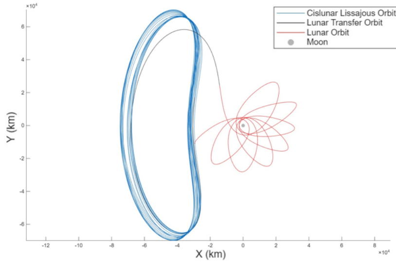
Figure 10: Artemis P2 trajectory in Earth-Moon synodic frame
