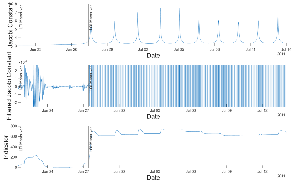
Figure 13: Artemis P1 orbit transfer maneuvers
