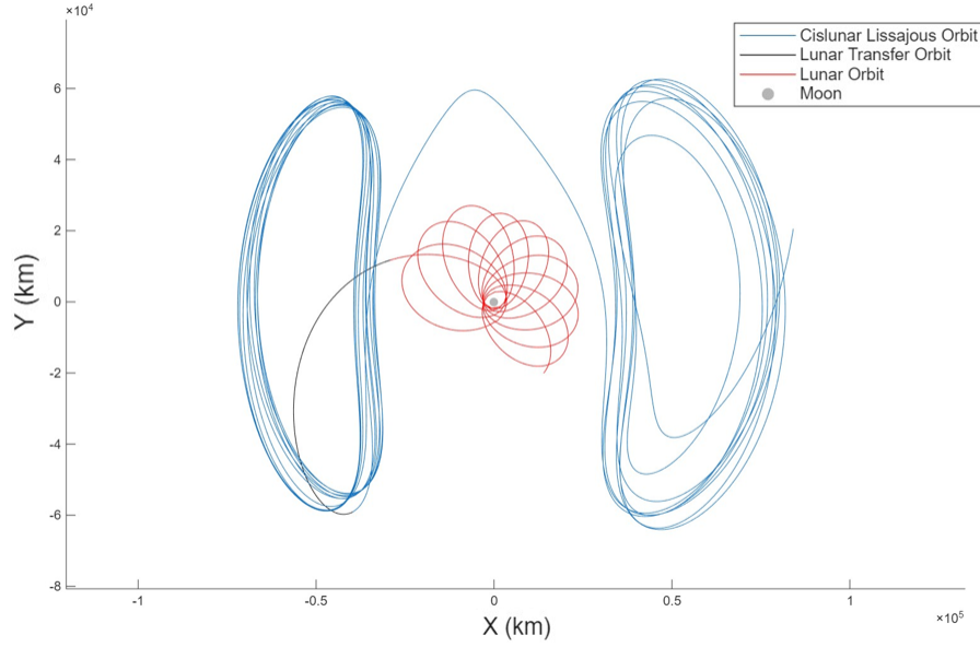
Figure 11: Artemis P1 trajectory in Earth-Moon synodic frame
