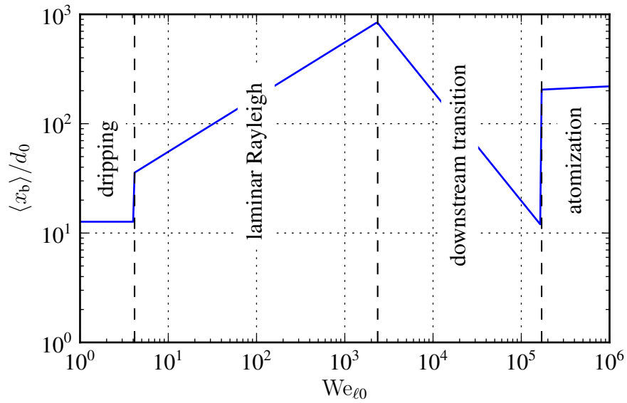
FIG. 8: Schematic “stability curve” for the pipe nozzle d_0 = 90 \mu\text{m} , n -dodecane (similar to Spray A but with a lower \text{Re}_{\ell 0, \text{crit}} ) case in figure 5. See figure 6 for details.
