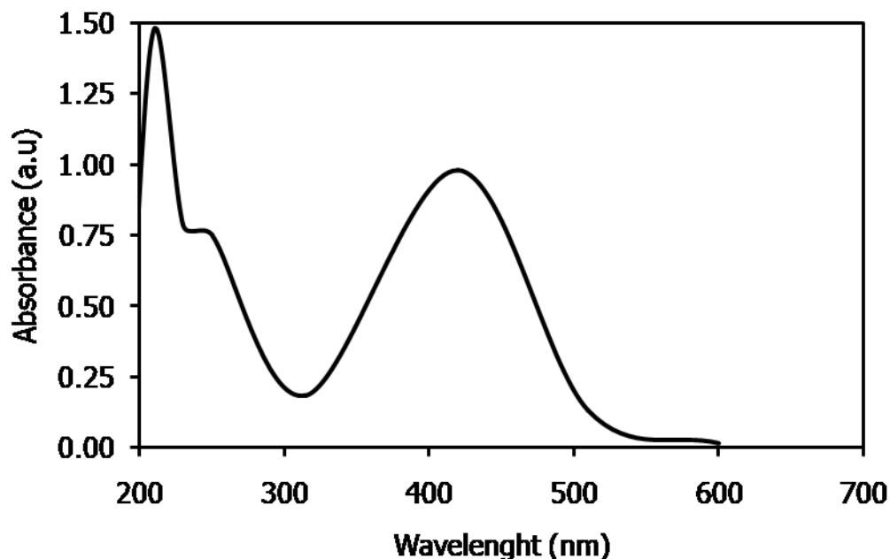
Fig.3 UV-Visible spectrum of experimental synthesis of AgNPs under optimum condition
