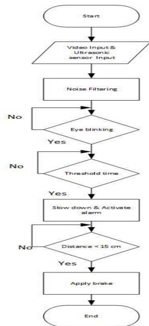
Figure 7 Flow chart of the design.
