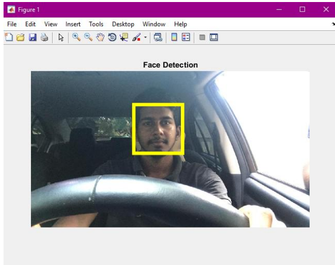
Figure 1 Face detection
