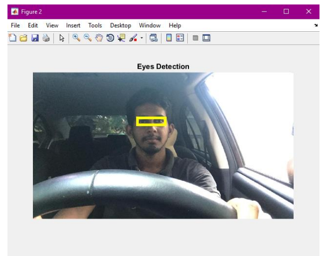
Figure 2 Eyes detection
