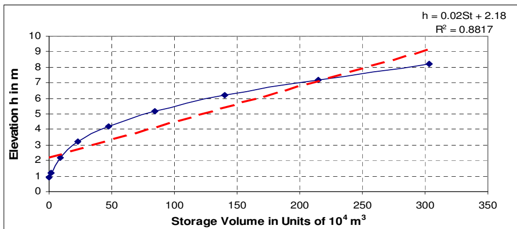
Figure 6.2 Storage-Elevation Curve
