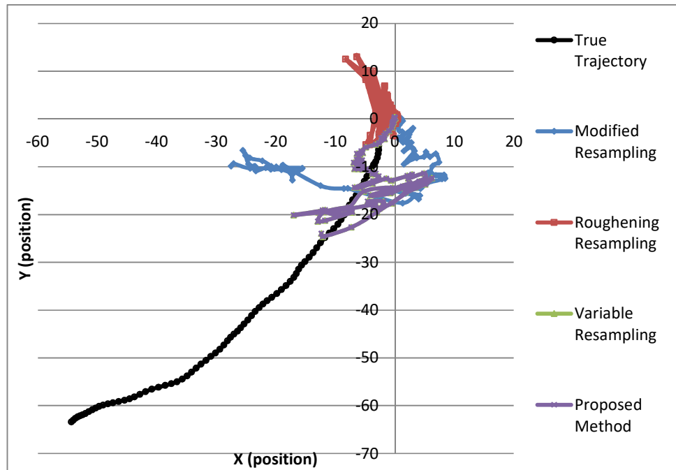
Fig. 10. Simulation of Particle Position Using Low Cost Inertial Sensor in Situation 3 (using 100 particle)
