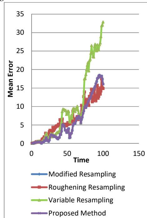
Fig. 6. Simulation of Mean Particle Error Using Lost Inertial Sensor in Situation 1..
