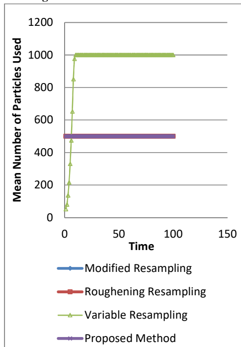
Fig. 5. Simulation of Mean Number of Particle Used Using Low Cost Inertial Sensor in Situation 1.
