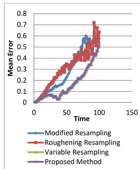
Fig. 15. Simulation of Mean Particle Error Using Lost Inertial Sensor in Situation 3 (using 10 particle)
