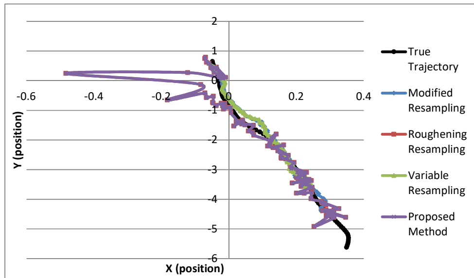
Fig. 7. Simulation of Particle Position Using Low Cost Inertial Sensor in Situation 2
