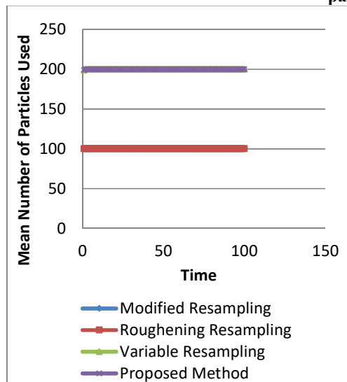
Fig. 11. Simulation of Mean Number of Particle Used Using Low Cost Inertial Sensor in Situation 3 (using 100 particle).
