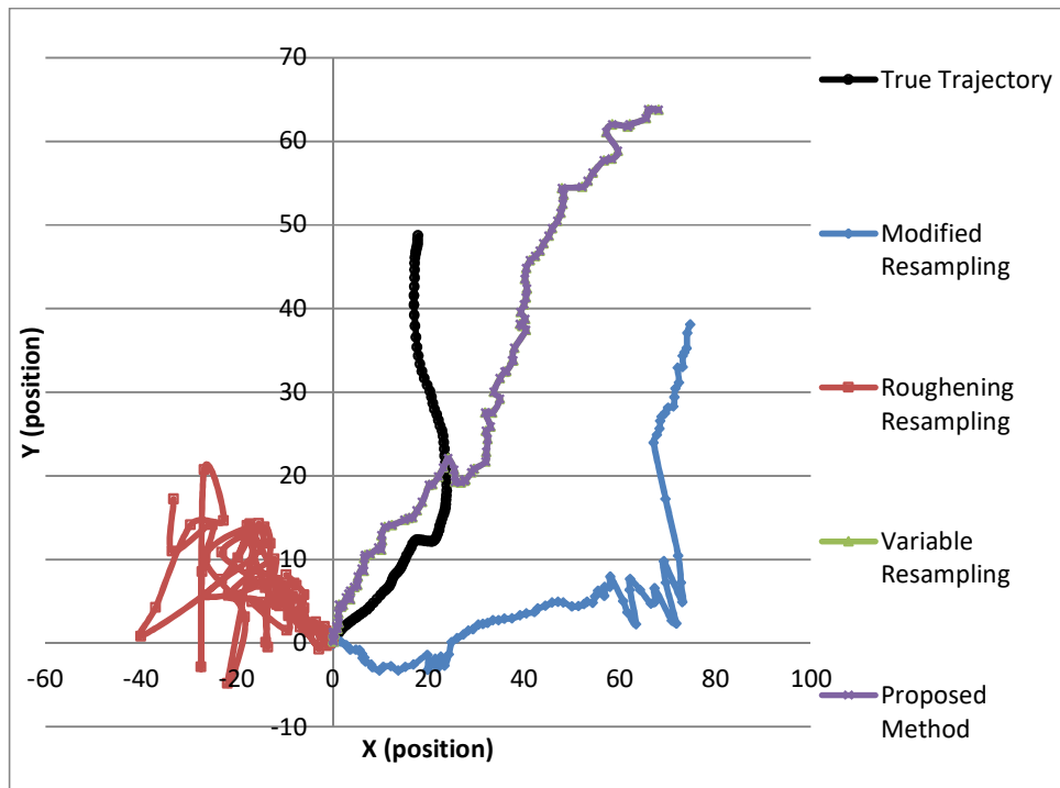
Fig. 13. Simulation of Particle Position Using Low Cost Inertial Sensor in Situation 3 (using 10 particle)
