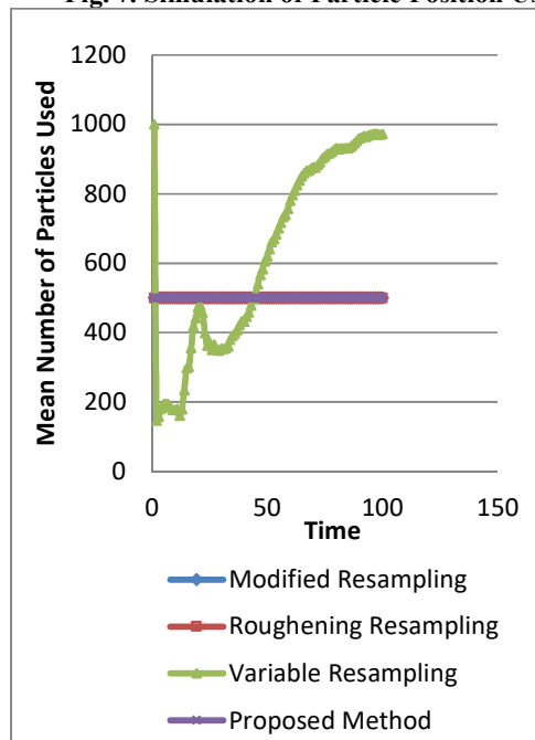
Fig. 8. Simulation of Mean Number of Particle Used Using Low Cost Inertial Sensor in Situation 2
