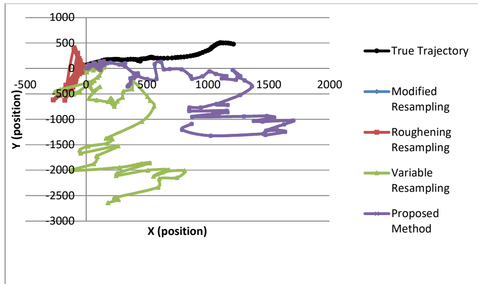
Fig. 4. Simulation of Particle Position Using Low Cost Inertial Sensor in Situation 1.
