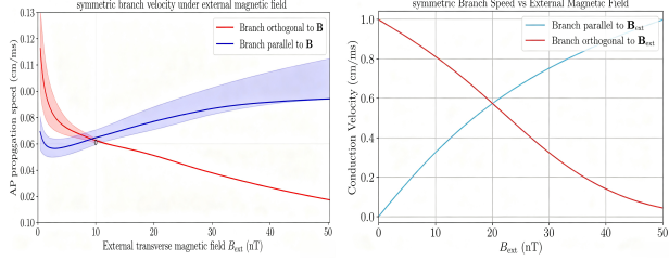
(c) Conduction speed for branches under transverse B . (d) Velocity response curve, symmetric crossover at B_{ext} = 20nT for parallel, orthogonal propagation symmetry.
