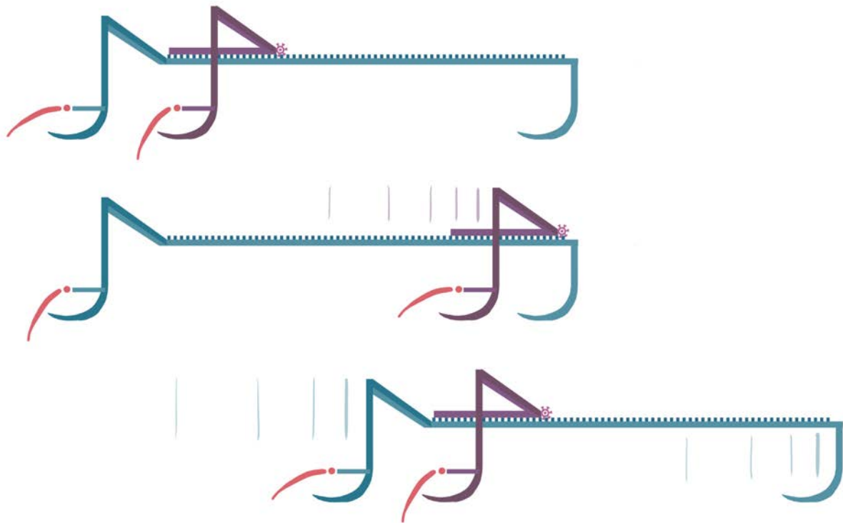
Fig. 2. The push phase of the UTOPUS motion cycle in lateral view. The vehicle moves from left to right. Note the two crampons in red attached to the back frame and the front frame (in purple). Note also that the shaft has an additional element in front of the purple frame for balance. This additional element has no effect on the traction mechanism. Top: At the end of a pull phase the front crampon is still anchored in the ground while the rear crampon is sliding over the ground. Middle: UTOPUS pushes the two frames apart. The front crampon has been pulled out of the ground and slides over the ground while its frame advances. The rear crampon has been pushed into the soil, firmly anchoring its respective frame. Bottom: UTOPUS pulls the two frames together again. The front crampon has anchored itself firmly in the ground. The rear crampon has been pulled out of the ground while its frame advances.
