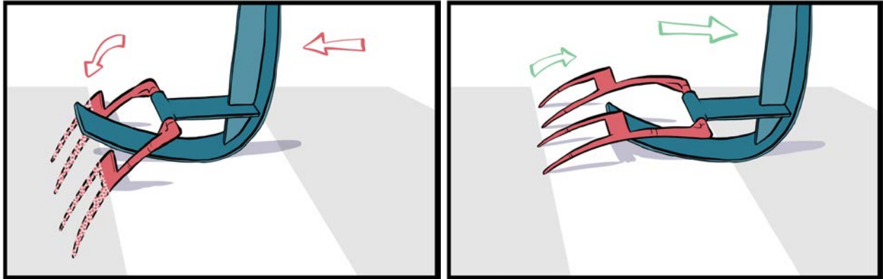
Fig. 1. The crampons are actuated by the motion of their respective frames. Left: When a frame is pushed backwards (in this illustration: to the left), its crampons are pushed into the ground in a circular motion. Right: When a frame is pulled forward (in this illustration: to the right), its crampons are pulled out of the ground and slide over the ground.
