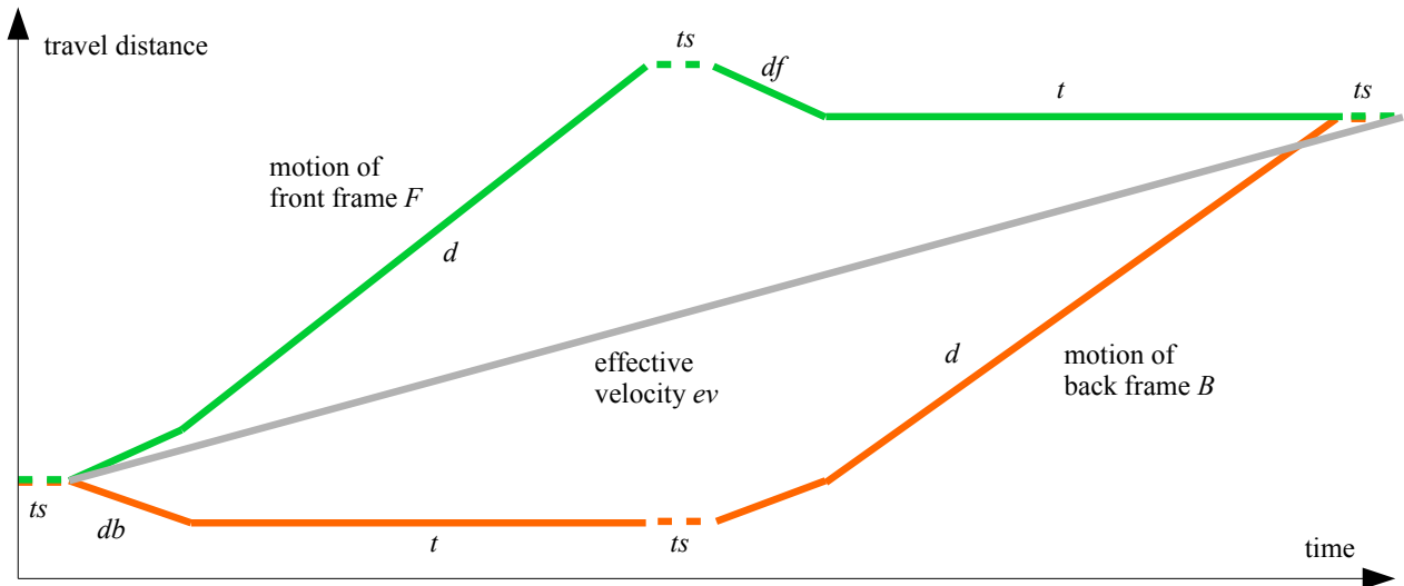
Fig. 4. Diagram of the motion dynamics of UTOPUS. The orange line illustrates the motion of back frame B and the green line illustrates the motion of front frame F. Note how the frames slip back by distances db and df at the start of a push or pull phase. During the time ts needed to switch the motor direction UTOPUS is almost at standstill.
