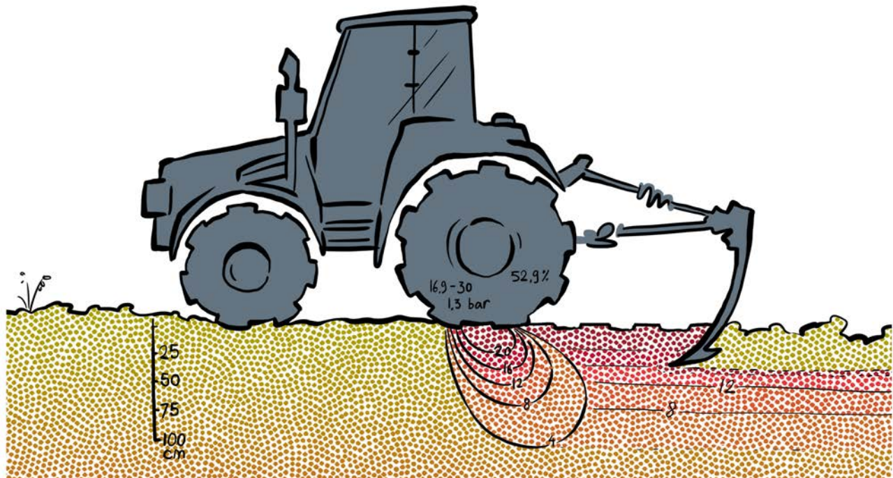
Fig. 1. The main axis of the pressure bulb under a tractor tire extends diagonally into the ground and compacts the soil below the depth of tillage (Söhne and Bolling, 1981).
