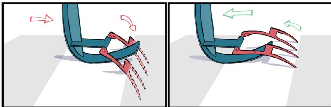
Fig. 5. Crampon placement can be implemented in a relatively simple way. The vehicle in this figure moves from right to left, such that when a frame is pushed or pulled back, it is moved from left to right. Left: The crampons are pushed into the soil. Right: the crampons are pulled out of the soil as the direction of travel is reversed.
