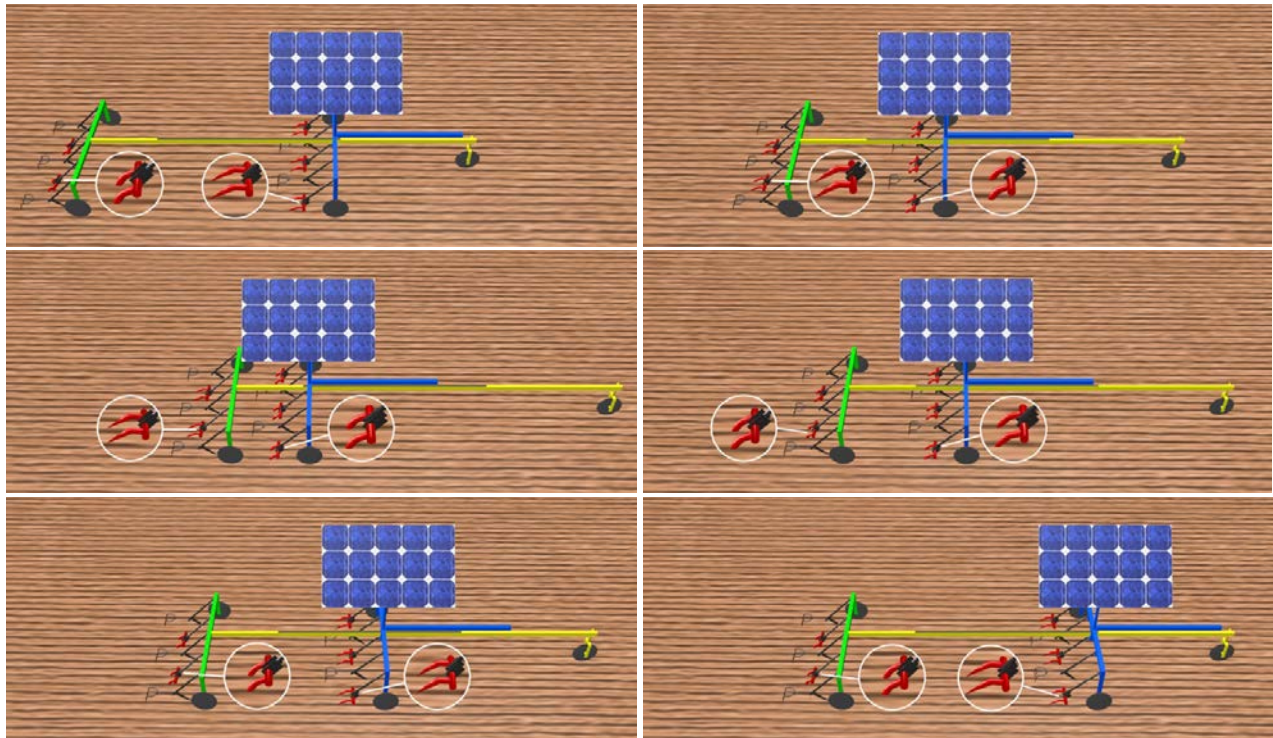
Fig. 6. Motion pattern of UTOPUS. The crampons on two frames are inserted and extracted from the soil in an alternating push-pull motion pattern. The crampons of one frame are always stable in the soil while the crampons of the other frame move together with its respective frame. The vehicle in this figure moves from left to right. Upper left: UTOPUS is fully extended. The left set of crampons are anchored in soil and the blue sliding frame is at the fully right position; Upper right: Right set of crampons are anchored in soil and left tillage tines are being pulled to the right; Middle left: At the end of the motion shown in upper right image UTOPUS has fully contracted; Middle right: Left set of crampons are anchored in soil and blue sliding frame with its tillage tines are being pushed to the right; Lower left: Continuation of motion in middle right image; Lower right: At the end of the push phase, UTOPUS is fully extended.
