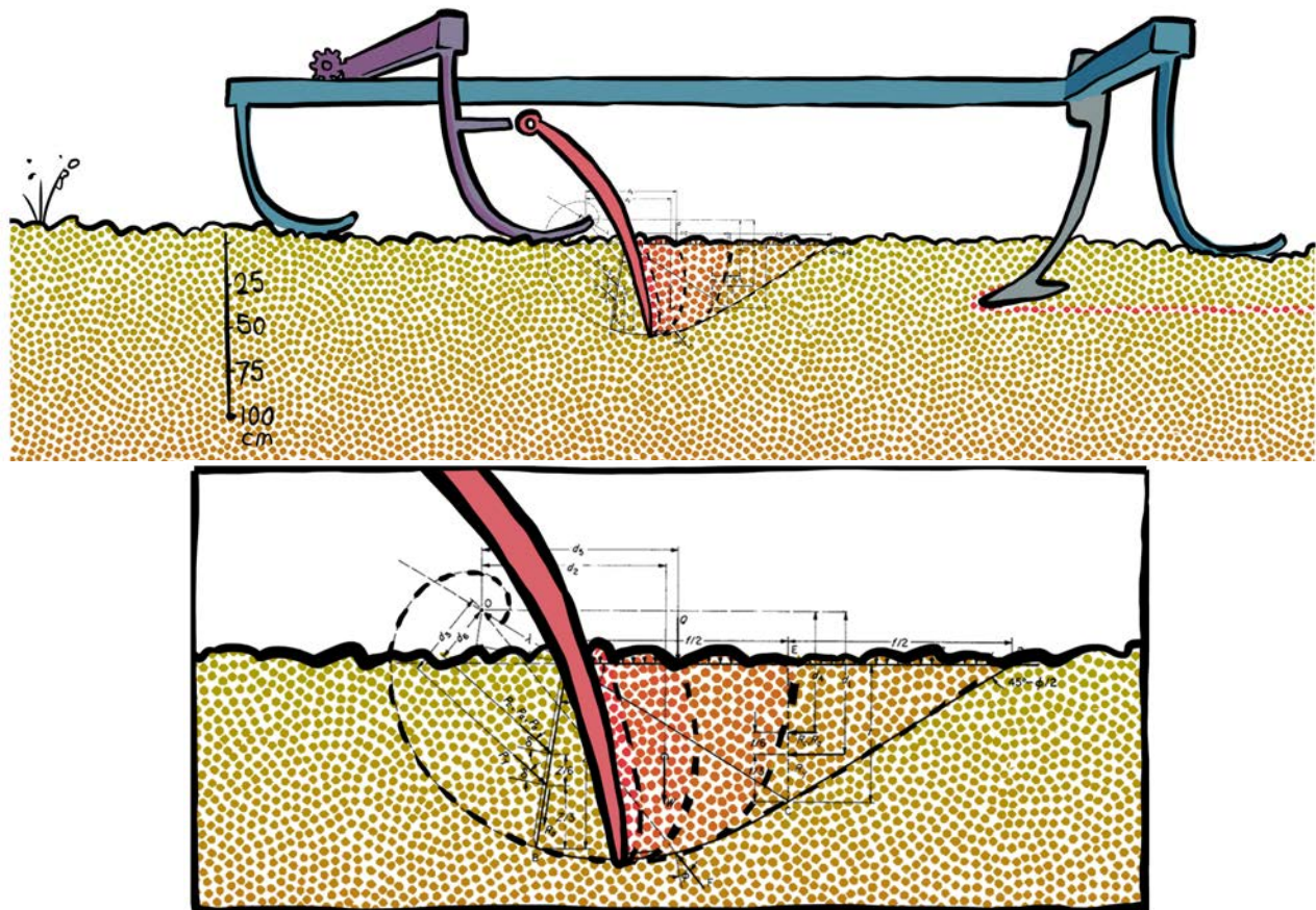
Fig. 4. A crampon pulls a plow with minimal compaction. In order to pull, crampons only need to press sideways into the soil, avoiding deep compaction. A curved crampon design helps the crampon to penetrate the soil and to reach an angle of close to 90^\circ from horizontal in the deeper soil layer, which maximizes soil resistance. The vehicle in this figure moves from right to left and the crampon pushes to the right.
