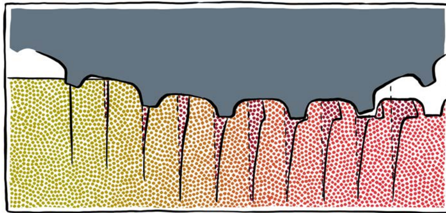
Fig 2. The horizontal shear force of the tire damages the soil just as much as the ballast (Söhne, 1952).
