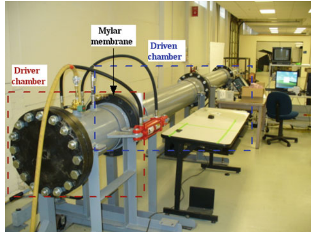
Figure 4 Shock Tube System at Wayne State, from Zhang [44] shared under CC BY 4.0
