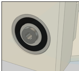
Figure 11: 609-series Ball-Bearing Slotted Into the Chassis to Stabilise the Rotary Shaft Piece
