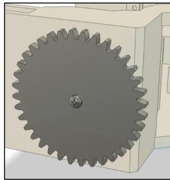
Figure 12: Spur Gear Screwed onto the Shaft with the Help of an M3 Threaded Heat Insert
