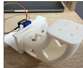
Figure 16: 3D-Printed Rotation Mechanism
