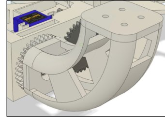
Figure 15: Drone Arm Fitted onto Chassis with Bearing and Meshed with the Rotation Gear
