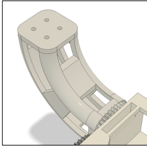
Figure 29: CAD Design of Drone Arm with Screw Holes for Motor
