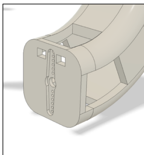
Figure 6: Engraving Into Arm to Directly Fit Servo Horn
