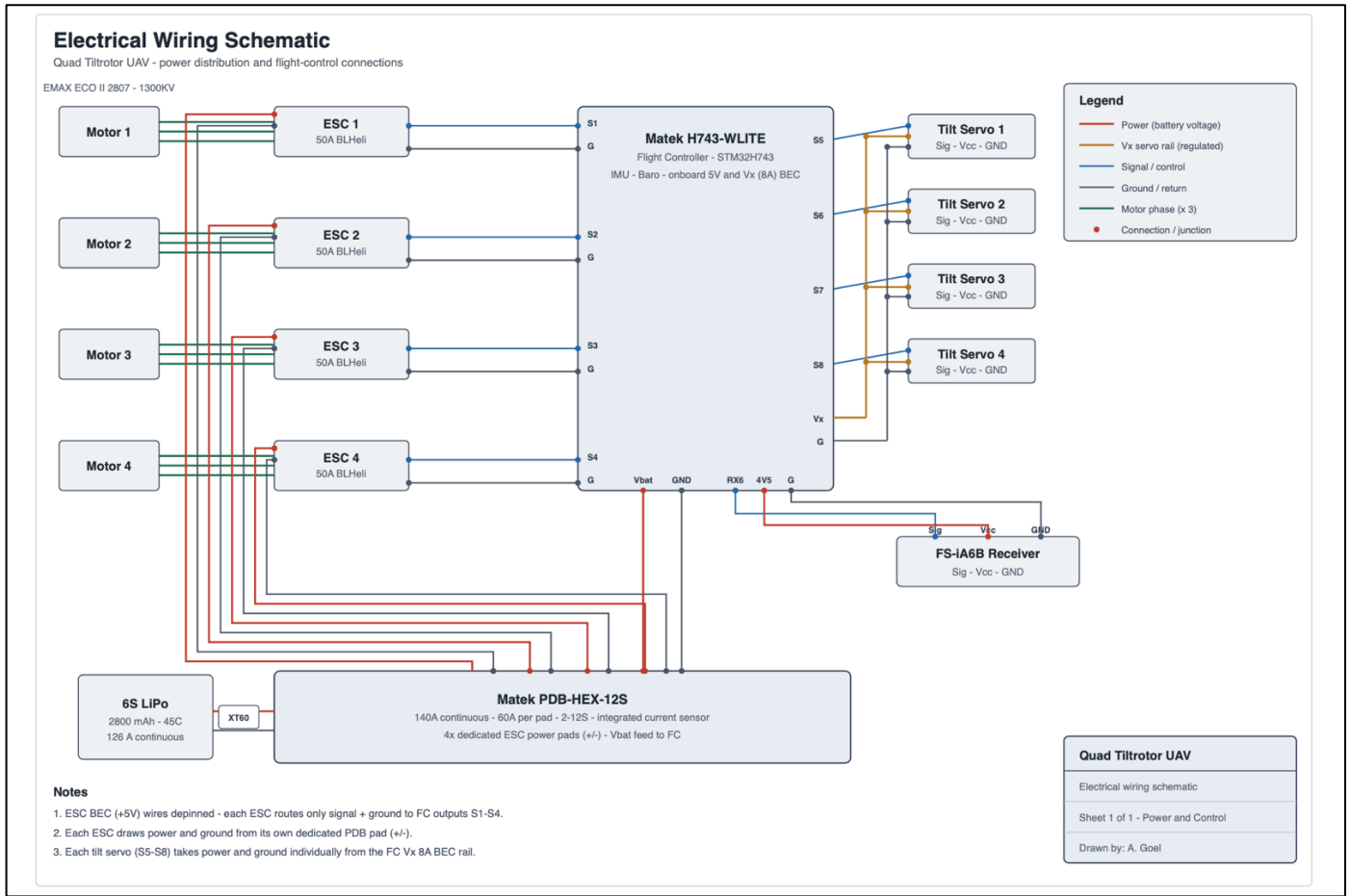
Figure 26: Electrical Wiring Schematic for the Circuit
