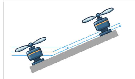
Figure 2: Side Profile of a Standard Quadcopter During Forward Motion; Blue Arrows Represent Airflow
