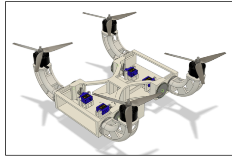
Figure 36: Completed CAD Design with some Components
