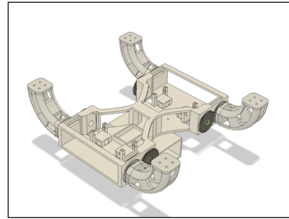
Figure 35: CAD Design Ready for Print (Without Components)
