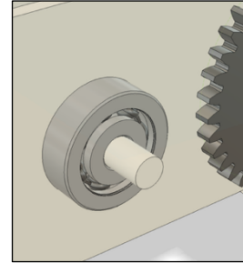
Figure 14: 635-series Ball-Bearing fitted onto Circular Beam
