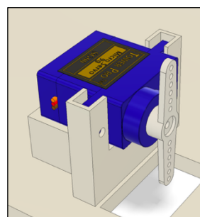
Figure 8: Servo Motor on Servo Stand
