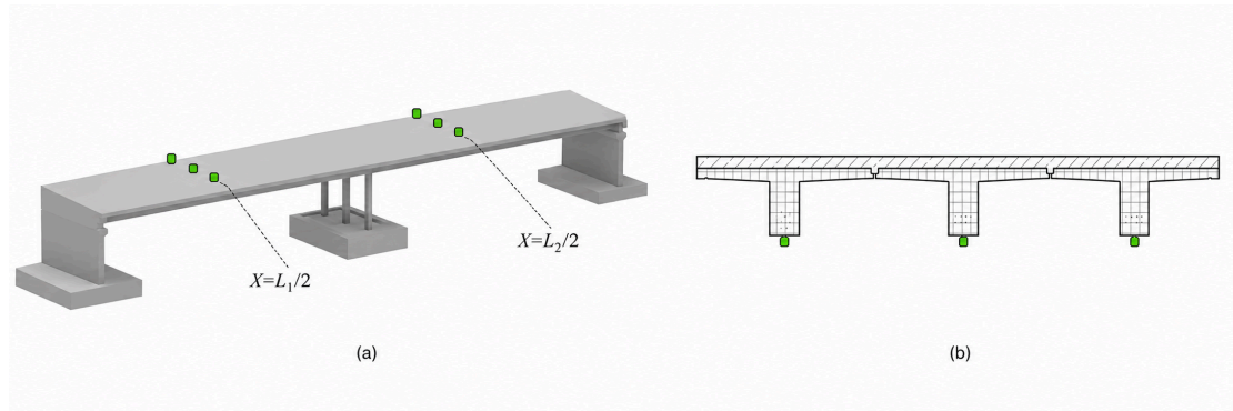
Figure 1: (a) Spatial topology and (b) cross-sectional piezoelectric accelerometer array of the openLAB reference bridge [1].
