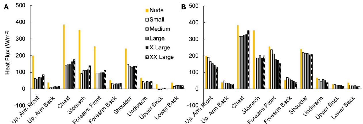
Fig. 5 Measured radiative net heat flux comparison across different shirt sizes for A. white and B. black long-sleeved shirts.
