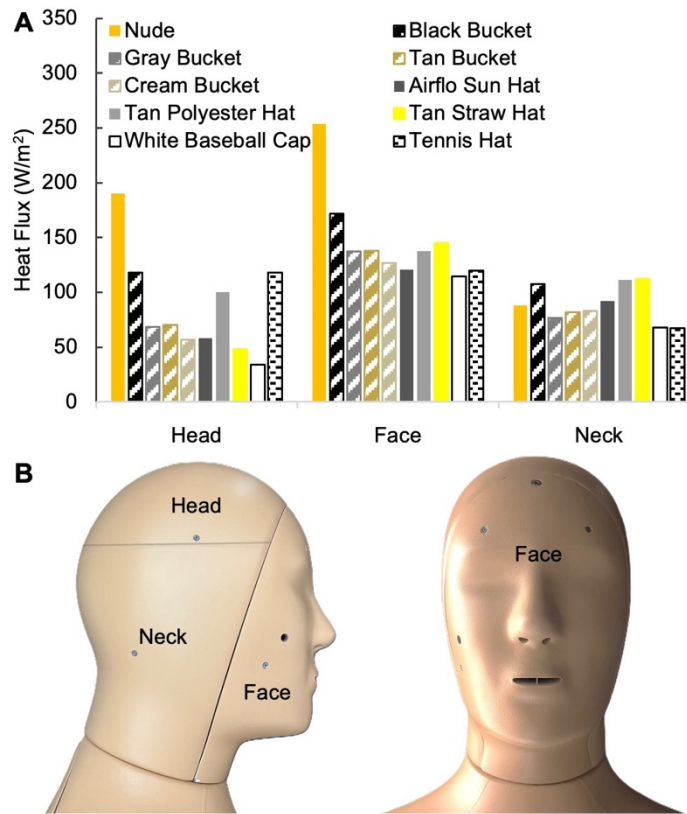
Fig. 7A. Comparison of radiative net heat flux measured across the head, face, and neck zones with a manikin wearing hats with assorted styles and colors, B. Images of the manikin showing the head, neck, and face zones.
