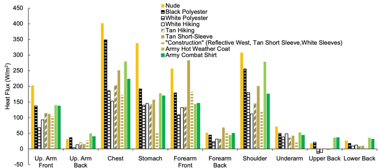
Fig. 6 Comparison of radiative net heat flux measured across upper body zones with a manikin wearing shirts with different styles and colors.
