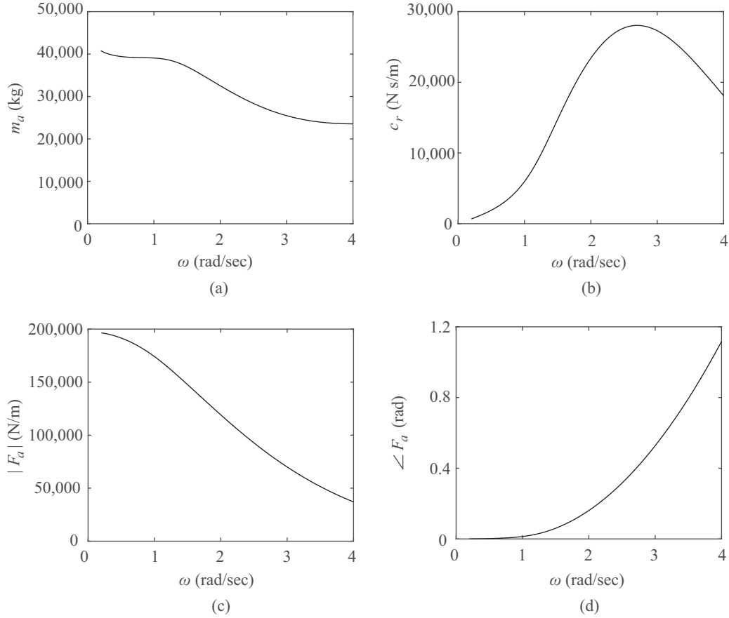
Figure 4: Hydrodynamic parameters for the heave mode of a circular cylinder with radius 2.5 m, draft 1 m, in water depth 30 m: (a) Added mass, (b) Radiation damping, (c) Magnitude of F_a(\omega) , (d) Phase of F_a(\omega) .
