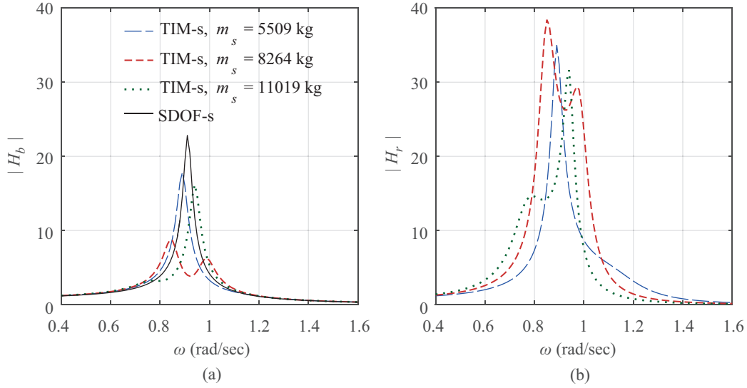
Figure 11: The amplitude of the transfer functions when the tuning spring stiffness is k_t^* = 6.06 \times 10^3 N/m and the damping coefficient C_{PTO} is set to the optimum value for T_p = 6 s: (a) H_b(\omega) , (b) H_r(\omega) .
