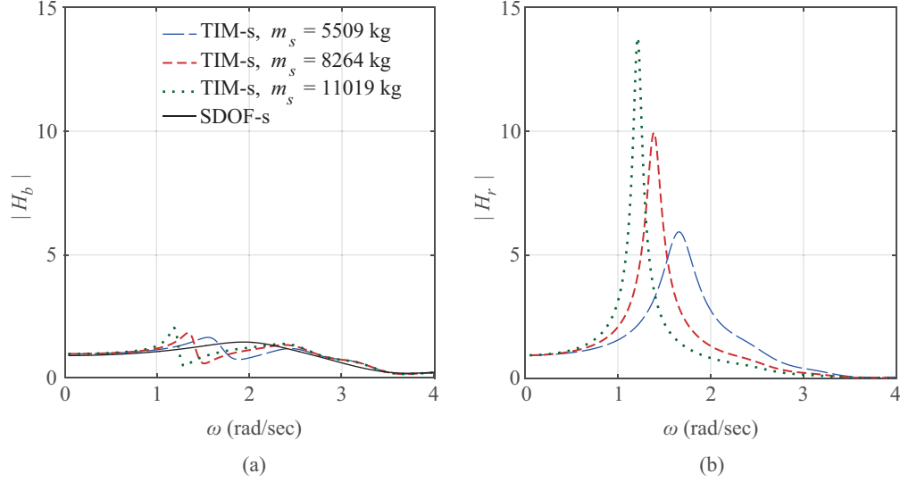
Figure 7: The amplitude of the transfer functions when the tuning spring stiffness is k_t^* = 1.72 \times 10^4 N/m and the damping coefficient C_{PTO} is set to the optimum value for T_p = 6 s, (a) H_b(\omega) , (b) H_r(\omega) .
