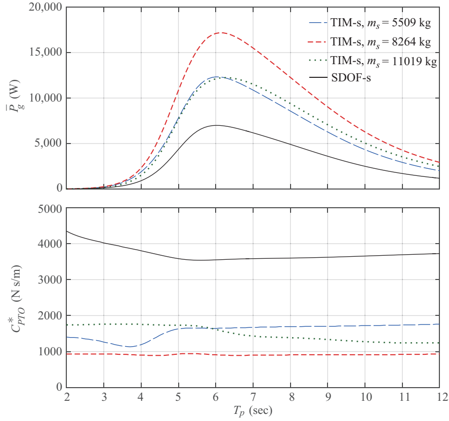
Figure 12: Power generation with phase control and optimum damping. For the TIM system, the tuning spring is set to k_t^* = 6.06 \times 10^3 N/m.
