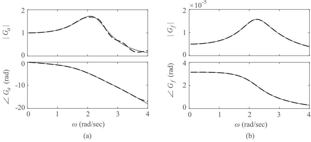
Figure 5: Frequency domain data (solid) and finite-dimensional approximation (dashed) with spatial delay of d = 10 m: (a) G_a(\omega) , (b) G_f(\omega) .
