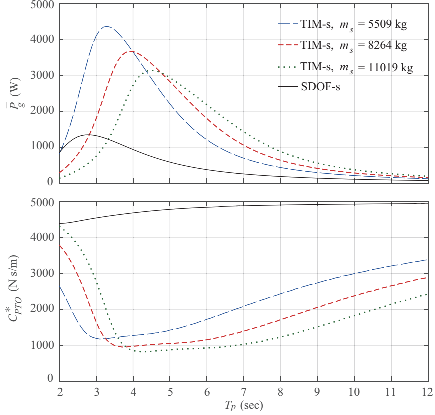
Figure 8: Power generation with optimum damping for each sea state. The tuning spring for the TIM system is set to k_t^* = 1.72 \times 10^4 N/m.
