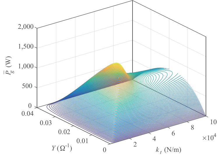
Figure 6: Contour plot of power generation showing the effects of the tuning spring stiffness k_t and admittance Y . The plots are for m_s = 8264 kg with sea state T_p = 6 s, H_s = 1 m, \gamma = 1 .
