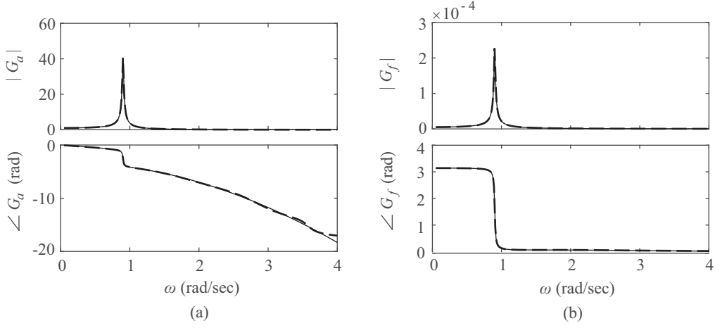
Figure 9: Frequency domain data (solid) and finite-dimensional approximation (dashed) with spatial delay of d = 10 m: (a) G_a(\omega) , (b) G_f(\omega)
