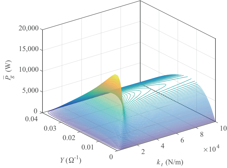
Figure 10: Contour plot of power generation showing the effects of the tuning spring stiffness k_t and admittance Y . The plots are for TIM system applied to a resonant buoy with m_s = 8264 kg and supplementary inertia of 200 t. Sea state is T_p = 6 s, H_s = 1 m, \gamma = 1 .
