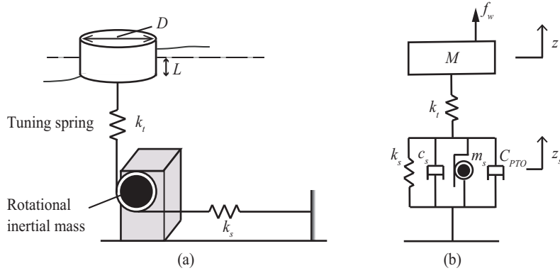
Figure 2: Point absorber with tuned inertial mass (TIM system): (a) Schematic illustration, (b) Model.
