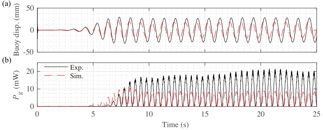
Figure 12: Comparisons of time histories of the experimental and simulation results for Type B-R2: (a) Buoy displacement, (b) Power generation.
