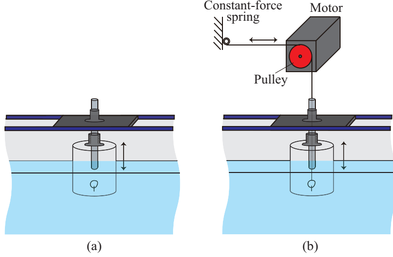
Figure 5: Decay test setup: (a) Buoy with the linear bushing, (b) SDOF WEC.
