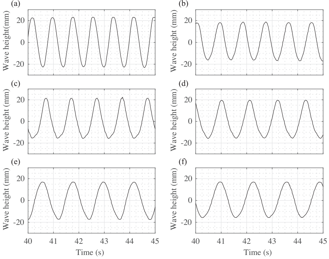
Figure 8: Wave height: (a) T_p = 0.8 s, (b) T_p = 0.9 s, (c) T_p = 1.0 s, (d) T_p = 1.1 s, (e) T_p = 1.2 s, (f) T_p = 1.3 s,.
