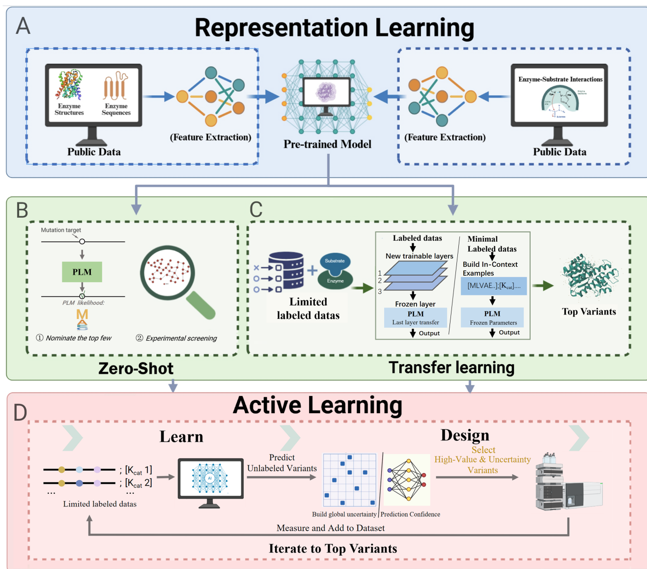
Figure 2. Architecture of few-shot machine learning methods. (A) Pre-trained models (e.g., protein language models) learn general feature representations from massive unlabeled sequence data or low-fidelity data, encoding sequence, structure, evolutionary, and functional information that can be transferred to downstream enzyme engineering tasks. (B) Pre-trained models are directly used as zero-shot predictors to assess the consistency of mutant sequences with the statistical patterns of natural sequences, enabling inference of mutational functional effects without experimental labeled data and allowing preliminary screening of promising mutants. (C) Transfer learning adapts pre-trained models to a target task using a small amount of experimentally labeled data, including parameter-efficient fine-tuning (PEFT) and in-context learning without parameter modification, significantly improving prediction accuracy compared with zero-shot methods. (D) A small subset is randomly sampled from a variant library for experiments, and a supervised model with uncertainty quantification is trained on the experimental data to predict the remaining unmeasured variants. An acquisition function is then used to nominate variants with both high uncertainty and high value, which are experimentally measured and fed back for retraining, iterating until top-tier variants are reached.
