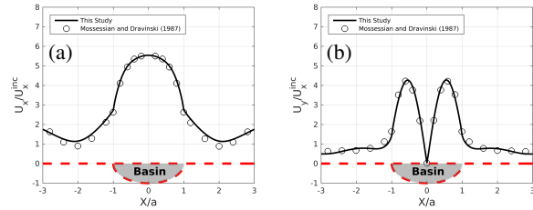
Figure 8. Surface AF in a) horizontal and b) vertical directions for semi-circular basin of Mossessian and Dravinski [32]
