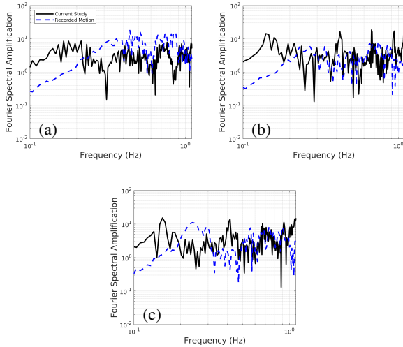
Figure 33. Comparison of simple HC basin (“Current Study”), and recorded motion during the mainshock from Takai et al (2016) [40] for a) TVU station b) PTN station and c) THM station
