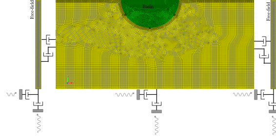
Figure 7. Schematic view of the FEM domain and boundary conditions.
