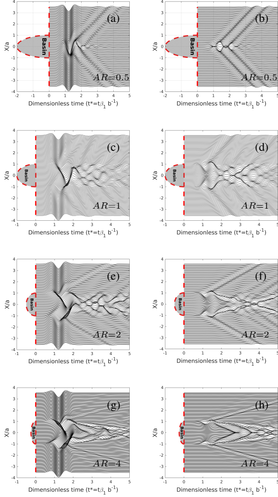
Figure 15. SS for AR = 0.5 (top panel), AR = 1 (second from top panel), AR = 2 (second from bottom panel) and AR = 4 (bottom panel) in a, c, e, g) horizontal and b, d, f, h) vertical directions. \eta = 1 and \beta_2/\beta_1 = 2 are assumed.
