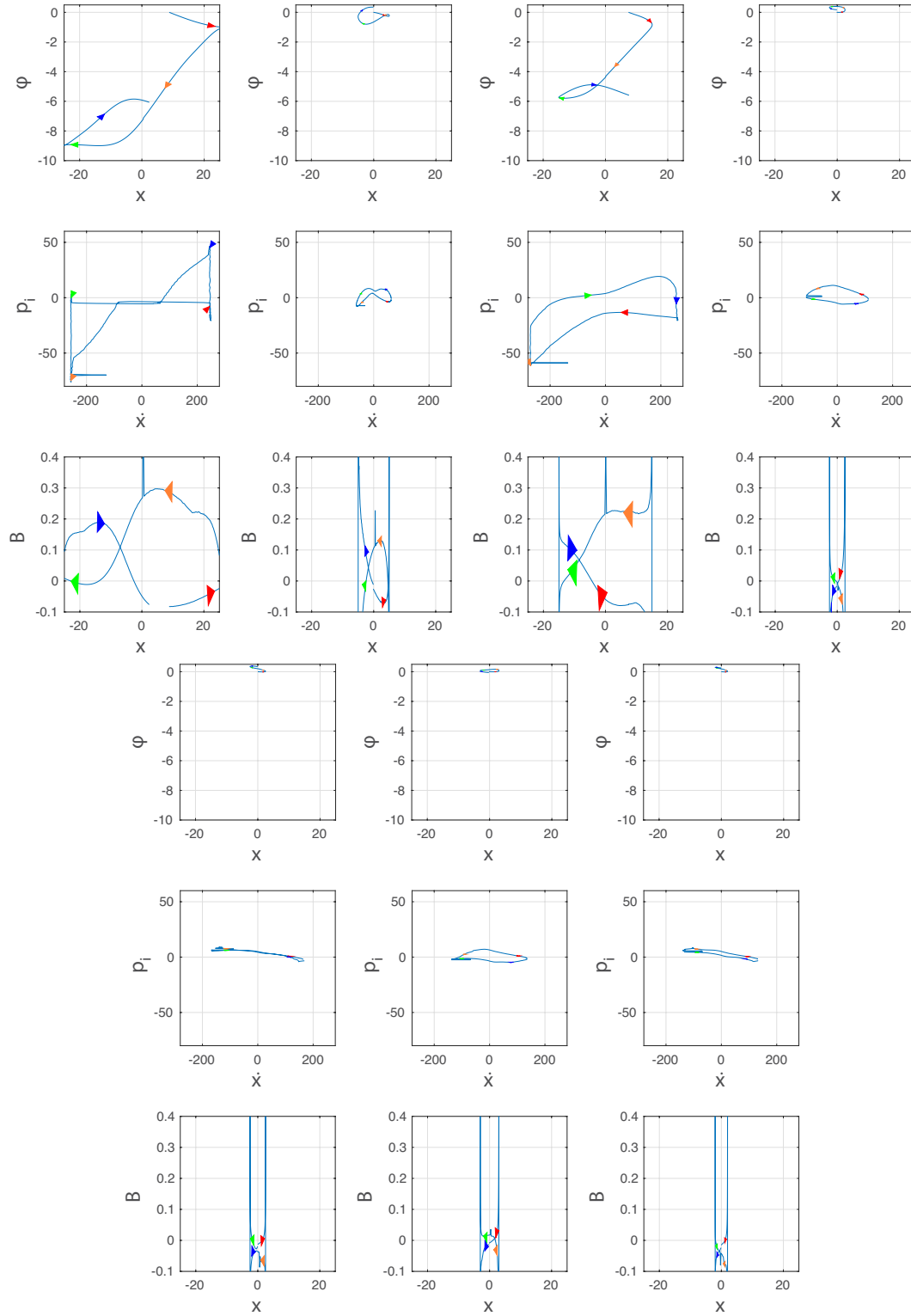
FIGURE 28 The approximated p_i = B(x)x for the mem-inerter component for a typical one cycle: Group 2 in Table 2. From top to bottom and left to right, they are: 30mm 2Hz, 5mm 2Hz, 15mm 3Hz, 2.5mm 7Hz, 2.5mm 10Hz, 3mm 7Hz, and 2mm 10Hz. Notice: There are physically meaningless portions
