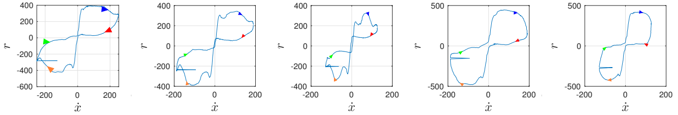
FIGURE 8 Useful loops of a typical one-cycle steady-state inerter response showing the origin-crossing behavior on the r vs \dot{x} plane in an approximate sense: Group 1 in Table 2. From left to right, they are: 20mm 2Hz, 15mm 2Hz, 10mm 2Hz, 10mm 3Hz, and 5mm 4Hz
