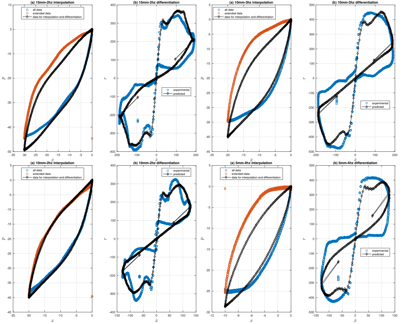
FIGURE 16 The experimental and predicted dual input-output pairs for the 15mm 2Hz, 10mm 3Hz, 10mm 2Hz, and 5mm 4Hz test in terms of (a) p vs x , and (b) r vs \dot{x} plots. In detail, the FFNN approximation and linear interpolation (see Fig. 15) were used to obtain the lower branch of p vs x , while the upper branch was placed by following the Masing's rule. The r vs \dot{x} was simply obtained by differentiating the time histories of p and x before combining them
