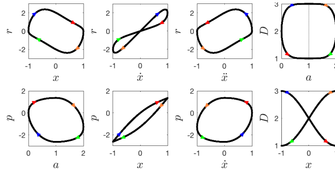
FIGURE 1 A particular mem-dashpot subject to the prescribed sinusoidal displacement input. For a linear dashpot, from the left to right columns, there would be ellipses, straight lines with a positive slope, ellipses, and constants of the value of the slope for D
