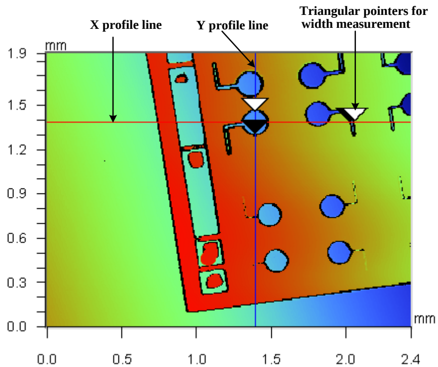
Figure 28. Topographic surface profile measurements of sample 2. The feature area is 2.4 mm x 1.9 mm.
