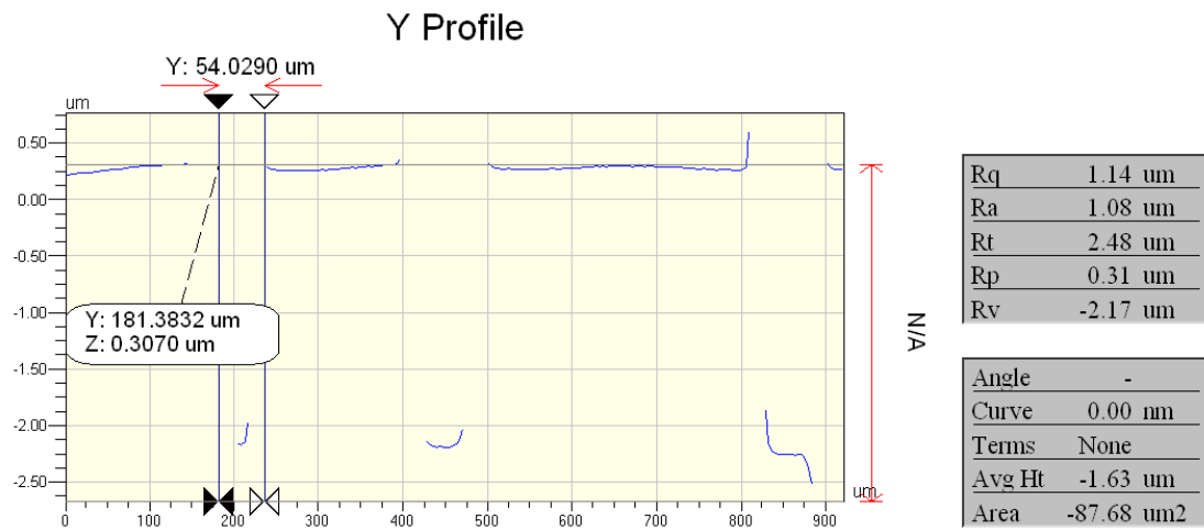
Figure 34. Y profile analysis of sample 3. The width of the horizontal line is about 54 μm.
