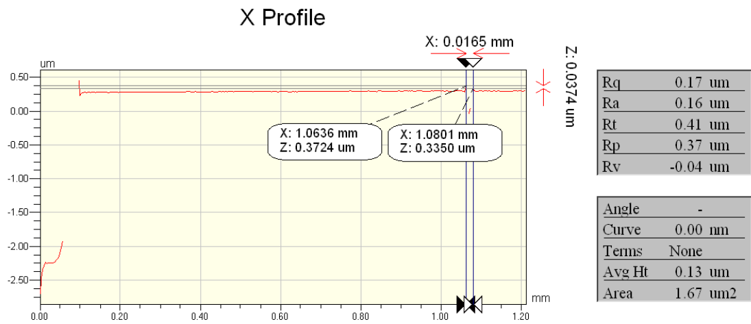
Figure 33. X profile analysis of sample 3. The width of the vertical line is about 17 μm
