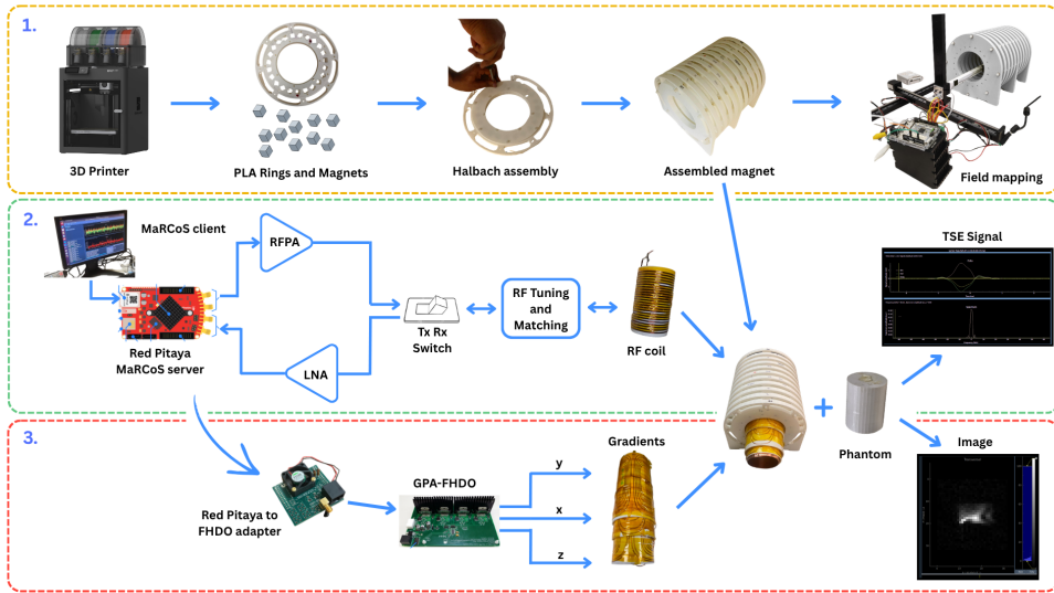
FIGURE 5 Steps to build an IMAGINE Scanner: 1) Print and assembly of the Halbach magnet, followed by field mapping with the three-axis robot. 2) Set up of RF chain to acquire a signal. 3) Integration of gradient circuit to acquire an image using a phantom. The Canada rat scanner components, signal and images are depicted here, but similar steps and components were used across sites to assemble the rat and mice/educational (ERNIE) scanner.
