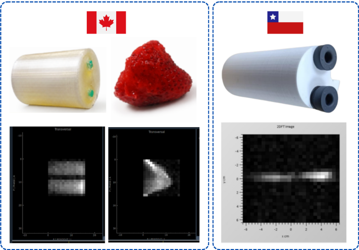
FIGURE 10 Phantoms and Spin Echo MR images acquired of those phantoms on the ERNIE scanners at the Canada (left) and Chile (right) sites.
