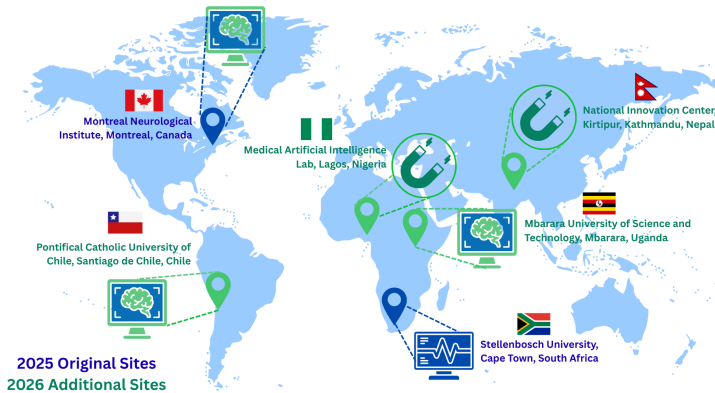
FIGURE 3 Build Laboratory Locations for the 2025 and 2026 programs, illustrating the resource-aware project expectations for each site. Two sites (Nigeria and Nepal) with no access to a local RF laboratory or MRI engineering infrastructure were tasked to assemble, disassemble, and reassemble their magnet and map the fields to investigate replicability. One site (South Africa) with emerging local MRI engineering infrastructure was tasked to generate the spin echo signal, while three sites equipped with standard RF labs and MRI engineering infrastructure generated a spin echo image for their build lab project.
