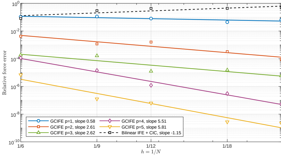
Fig. 6: Single-particle field-gather error against the common analytic kernel-average reference on N = 6, 9, 12, 18, 24 . The bilinear-IFE control uses four-node CIC with a centered-difference nodal field; GCIFE p = 1, \dots, 5 uses the fixed compact kernel. The particle position is fixed. Markers are computed errors and lines are five-mesh log-log fits. The CIC fit is negative in this mesh range, and the method-dependent gathering operators are specified in the text.
