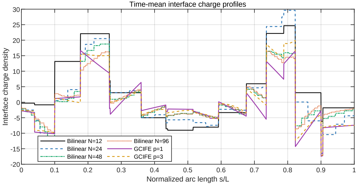
Fig. 8: (a) Mean interface charge density along normalized arc length for bilinear IFE–PIC at N = 12, 24, 48, 96 and the GCIFE–PIC p = 1, 3 results. Profiles are shown without smoothing.
