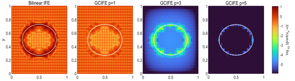
Fig. 3: Pointwise absolute gradient error for the elliptical-interface problem on the 24 \times 24 mesh. Panels show bilinear IFE and GCIFE degrees p = 1, 3, 5 using a common logarithmic color scale. The white curve is the exact interface. Integrated potential and field errors and refinement fits appear in Figure 2.
