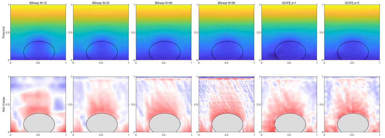
Fig. 7: Mean potential (top) and signed net charge density (bottom) on the common 96 \times 96 display grid. Columns show bilinear IFE-PIC/Boris at N = 12, 24, 48, 96 , followed by the GCIFE-PIC p = 1 /Boris and p = 3 /Boris-SDC4 results. The ellipse marks the true dielectric interface, and the gray region is the dielectric.
