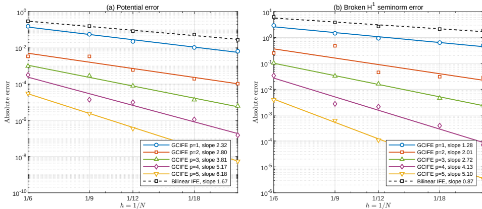
Fig. 2: Elliptical-interface convergence for bilinear IFE and GCIFE degrees p = 1, \dots, 5 on five meshes: (a) L^2 potential error and (b) broken H^1 seminorm error.
