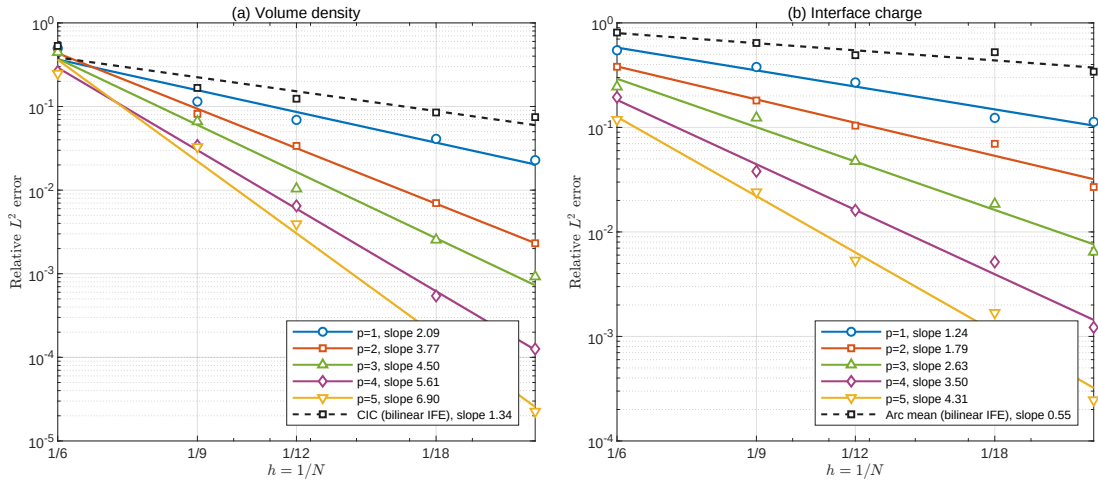
Fig. 4: Relative L^2 density errors for classical deposition controls and GCIFE degrees p = 1, \dots, 5 on N = 6, 9, 12, 18, 24 . (a) Volume density, using CIC for the bilinear-IFE control and a particle lattice refined alongside the mesh. (b) Interface charge, using segmentwise arc-length averages for the control, for one fixed group of six events, with unchanged physical positions, charges, and kernel on every mesh. Markers show computed errors and lines show five-mesh log-log fits. Charge conservation is stated in the text.
