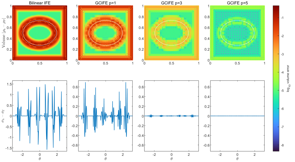
Fig. 5: Spatial density errors at N = 24 . The bilinear-IFE column uses CIC for volume charge and segmentwise arclength averages for interface charge. The remaining columns show GCIFE degrees p = 1, 3, 5 . The top row displays |\rho_h - \rho_p| for the source-refined particle lattice at fixed cell-interior points with a common logarithmic color scale. The white curve is the exact interface. The bottom row displays the signed difference \sigma_h - \sigma_\varepsilon along the interface parameter \theta , with a separate scale for the bilinear control and a common scale for the GCIFE panels. The bottom row uses the same fixed six-event group as Fig. 4. Integrated errors appear in Fig. 4(b).
