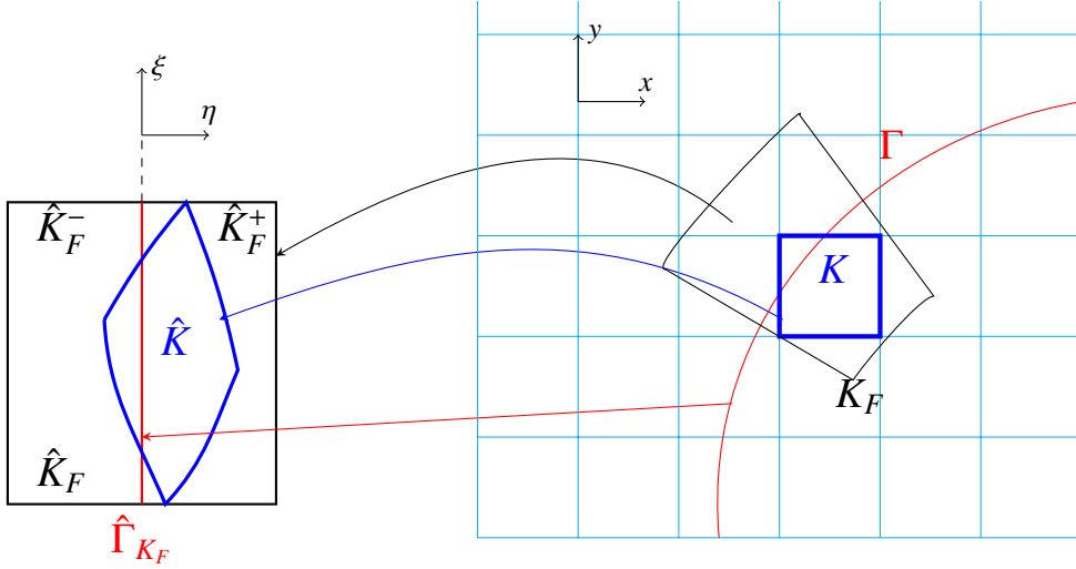
Fig. 1: Schematic of the Frenet mapping. Right: In the physical (x, y) domain, the Cartesian cell K is intersected by the curved interface \Gamma , enclosed by a fictitious Frenet box K_F . Left: The inverse mapping R_\Gamma transforms K_F into a standard rectangle \hat{K}_F , where the exact curved interface is straightened into a linear segment \hat{\Gamma}_{K_F} along the \xi -axis, precisely embedding the curvature physics into the local metrics.
