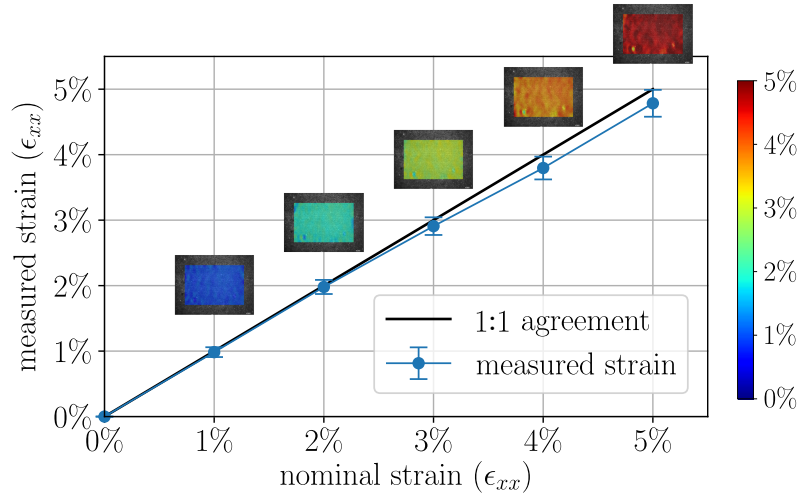
Figure 10: Results from uniaxial tension experiments with a polymer band specimen between nominal strains of 10,000\text{ }\mu\epsilon (1%) and 50,000\text{ }\mu\epsilon (5%). Error bars represent one standard deviation of the calculated strain values over the DIC region of interest. All strains are Green-Lagrange.
