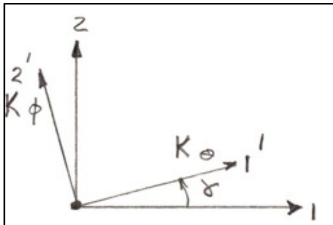
Figure 2. Principal stiffness-axis orientation used to introduce bending-torsion cross-coupling into the swept-wing structural model.
