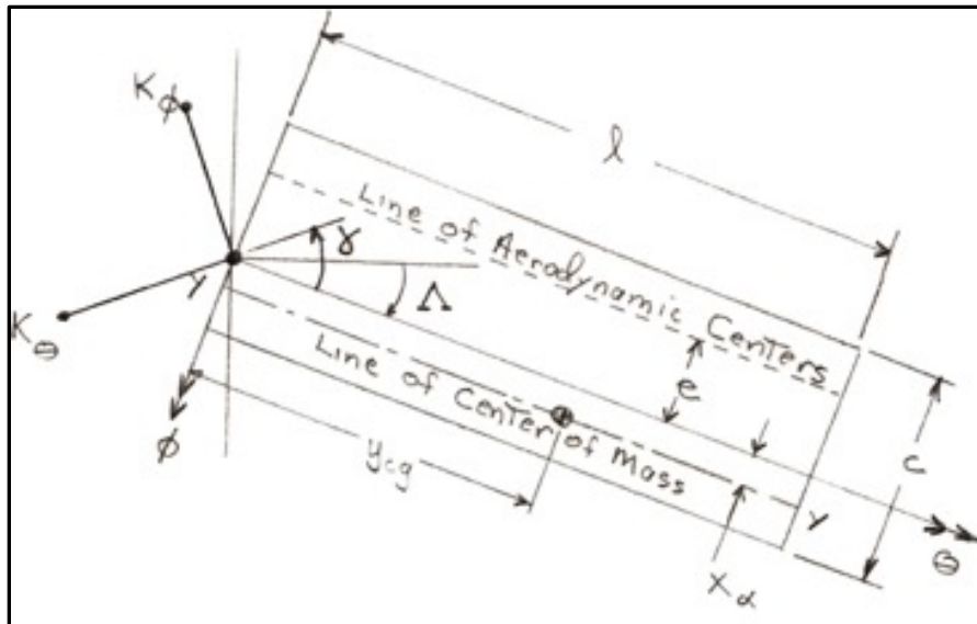
Figure 1. Idealized swept lifting-surface model showing how torsional and bending rotations are defined about the reference-axis attachment point.
