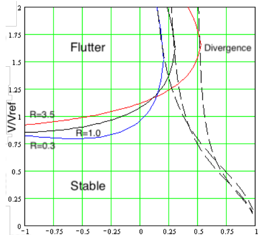
Figure 4. Corrected Mathcad results for \Lambda = 15 \text{ degrees} predict flutter and divergence boundaries that vary systematically with stiffness cross-coupling; the divergence curves intersect the corresponding flutter curves for the same torsional-to-bending stiffness ratio.
