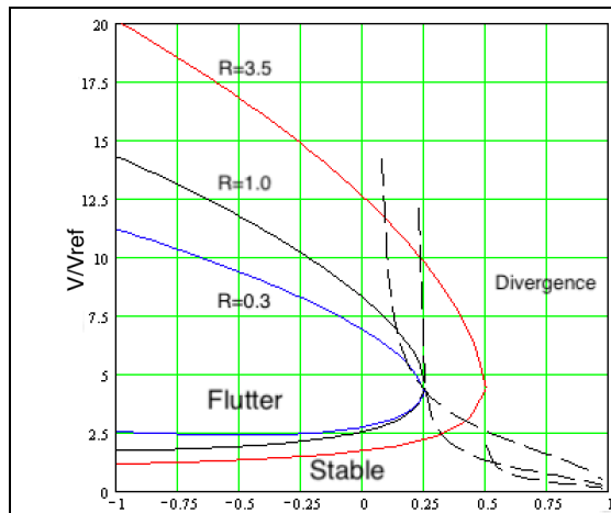
Figure 5. Using the original Journal of Aircraft equations for a sweptback wing in Mathcad shifts the computed flutter and divergence velocity curves, demonstrating the errors for \Lambda = 15 \text{ degrees}
