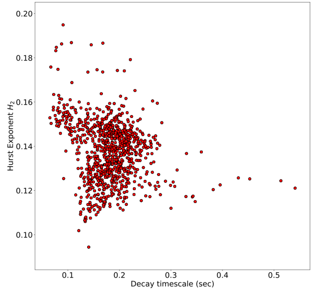
FIGURE 10. PLOT OF GENERALIZED HURST EXPONENT H_2 VS DECAY TIMESCALE
