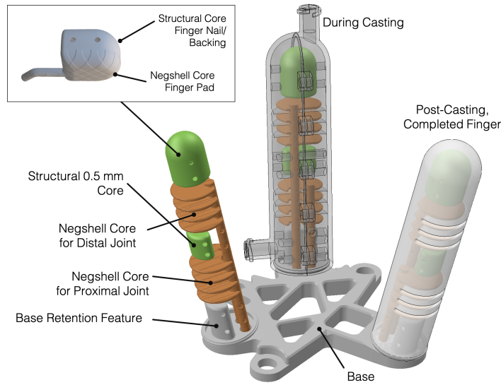
Fig 15. Overview of three-finger gripper's fabrication. The 3D-printed base, which serves as a part of the mold for the fingers, provides a rigid connection from the fingers to the tool plate of the WAM Arm. Two separate negshell cores are used for each joint of the fingers. A structural core aids in rigidity and force transmission between the joints. The fingertip contains a hybrid structural-negshell core with renders a soft finger pad and solid backing, as shown in the inset. The base also contains a retention feature geometrically similar to the structural cores, where silicone will be mechanically trapped and locked in place due to the overhang.
