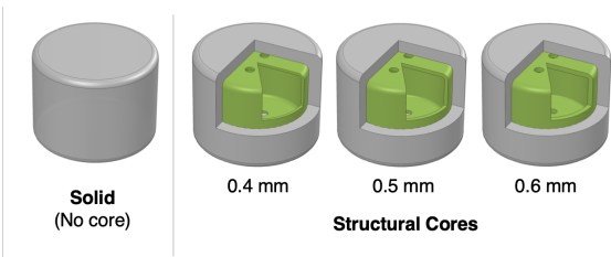
Fig 9. Structural core specimens. The four types of strutural core silicone specimens tested. The solid specimen has homogeneous material throughout its volume. The cores in the other specimens have a thickness of 0.4 mm, 0.5 mm, and 0.6 mm.
