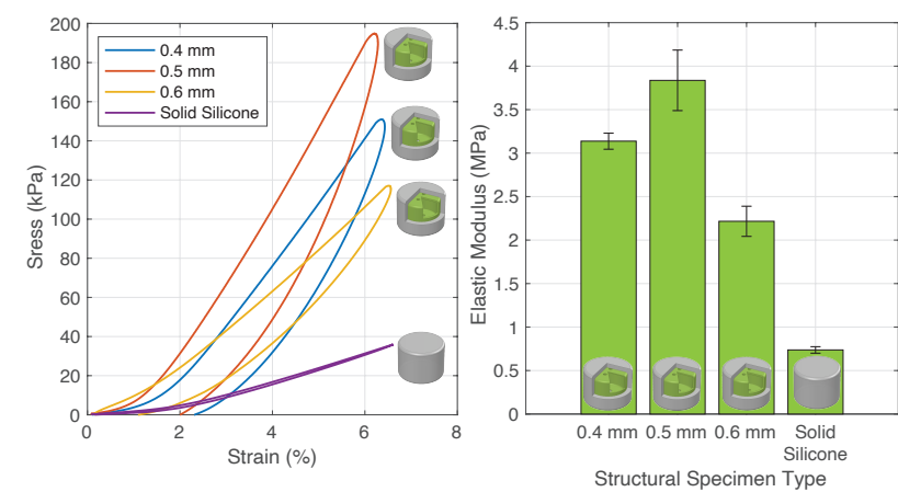
Fig 13. Structural core results. (Left) The stress-strain curve of the tested specimens show that the stiffness of the specimens can be greatly increased with the structural cores. (Right) The elastic modulus of the different structural cores.
