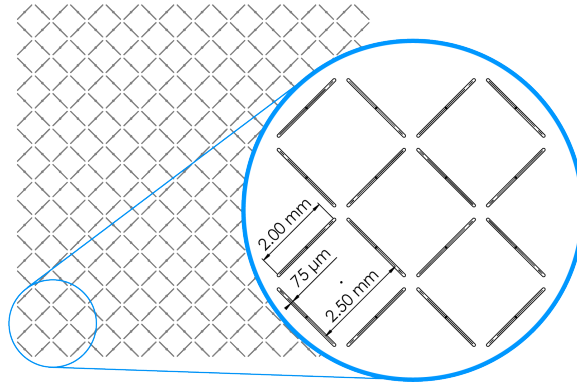
Fig 2. Cross-hatch pattern for perforating negshell cores. The cross-hatch are 75 \mu\text{m} wide by 2 mm long slots oriented in a 2.5 mm by 2.5 mm square pattern. The slots are designed to be small enough to be partially fused during printing to keep geometric integrity but also become fragile under load.
