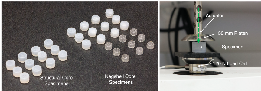
Fig 7. Experimental setup. (Left) All of the specimens used for testing. (Right) The specimen is placed at the center of the platen. As the actuator moves the platen down, the specimen is compressed and the resulting force is read from the load cell beneath.
