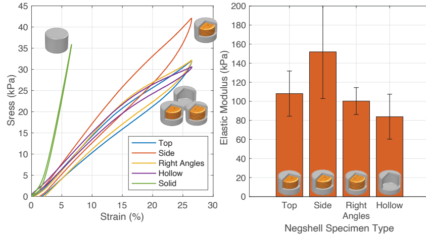
Fig 12. Negshell cores results. (Left) The stress-strain curve of the tested specimens show that the negshell cores minimally effect the mechanical property of the specimens under compression. The stress-strain curve of a solid, homogeneous specimen is also plotted as reference. (Right) The elastic modulus of the tested specimens.
