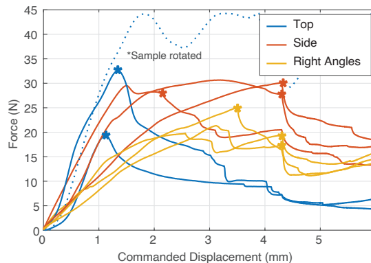
Fig 11. Breaking force for negshell specimens. Each specimen required different amounts of force to start rupturing, as denoted by the asterisks that precedes a sharp decline in force reading.
