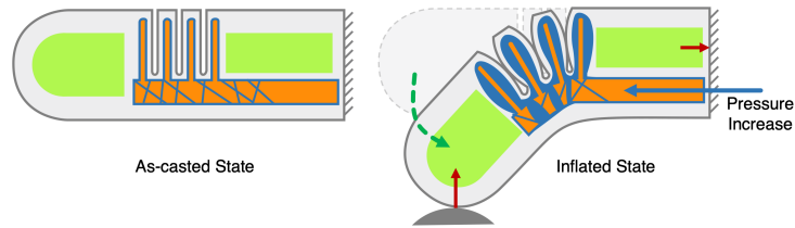
Fig 6. Main actuation principle of the soft robotic finger. As the actuation fluid (air/water) increases in pressure or volume, the fluid travels along the cavity left by the negshell core up to the fins of the bellows and start to expand the thin walls of the silicone elastomer surrounding the fins which creates a bending force.
