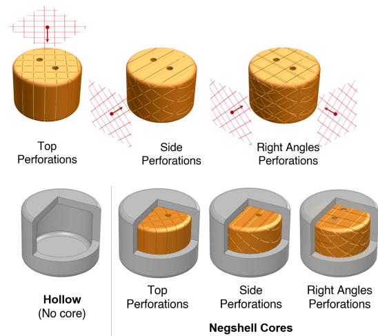
Fig 8. Negshell core specimens. The four types of negshell core silicone specimens tested. A zonal cross-section shows the internal features of the specimens. The hollow specimen does not contain any core. The negshell core specimens contain the three different cores with different perforation directions.
