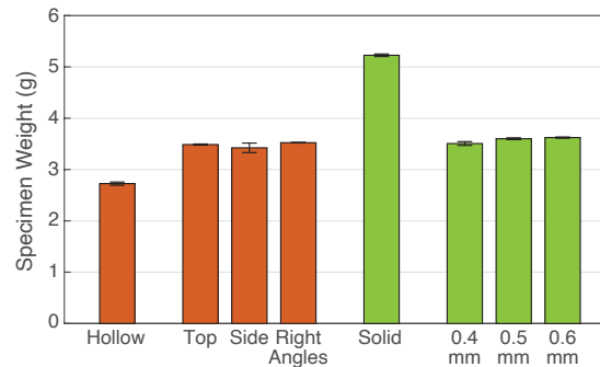
Fig 10. Specimen weights. Three samples of each type of specimen was weighed on a 0.01 gram resolution scale and averaged. The errorbars represent the standard deviation.
