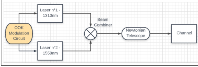
Fig. 2. System architecture for two wavelength optical link.
