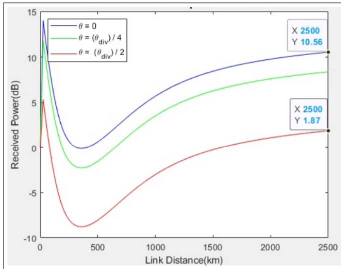
Fig. 4. Received power for the 1550nm link.
