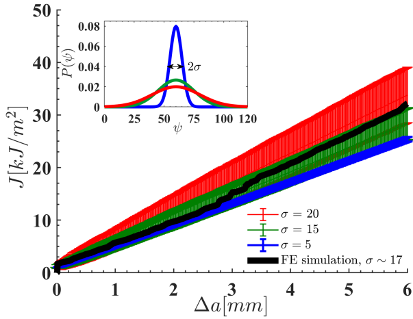
Fig. 8 The 95% confidence envelope for the crack growth resistance curves of a grain boundary network with a facet length of da = 160\mu\text{m} and a Gaussian distribution of deflection angles with a mean of \Psi = 60 and a standard deviation of: \sigma = 5 (blue); \sigma = 15 (green); \sigma = 20 (red). The results of a FE simulation for a grain microstructure with the same average facet length and \sigma = 17 is shown for comparison (black).
