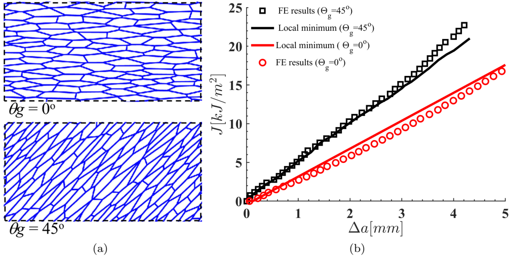
Fig. 7 (a) The elongated grain microstructure with an aspect ratio of 1:5 and rotated at an angle of \theta_g = 0^\circ and 45^\circ with respect to the crack growth direction. (b) Comparison of the crack growth resistance curves obtained using the microstructure-based finite element calculations and predicted using the proposed model when following the path of local minimum crack growth resistance for the two microstructures.
