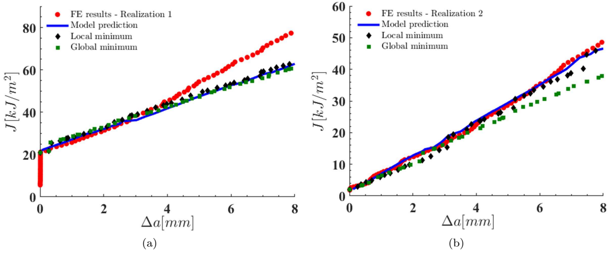
Fig. 4 Comparison of crack growth resistance curves obtained from the microstructure-based finite element calculations (FE results) and predicted using the proposed model when following the same crack path as obtained from the finite element calculations (Model prediction), when following the crack path of global minimum crack growth resistance (Global minimum) and when following the path of local minimum crack growth resistance (Local minimum) for two realizations of the specified grain microstructure: (a) realization 1 and (b) realization 2.
