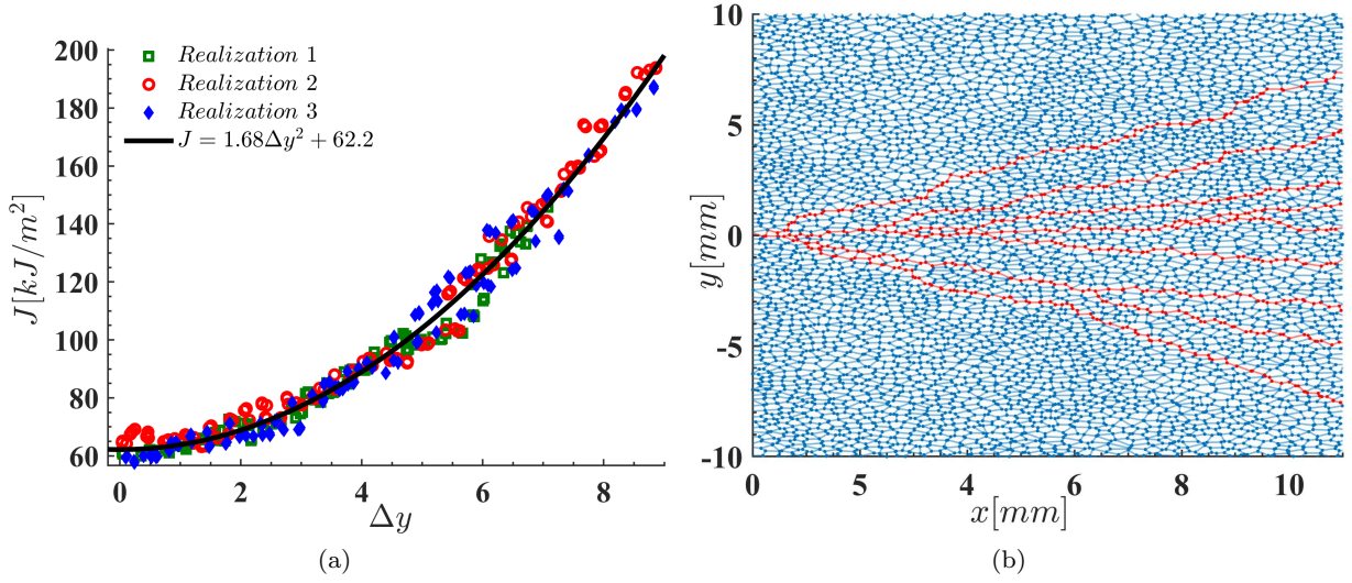
Fig. 6 (a) The dependence of overall crack growth resistance, J , for a specified amount of projected crack extension, \Delta a , along the crack propagation direction ( x -axis) on the overall crack deflection, \Delta y , from the crack propagation direction for three realizations of a specified grain microstructure. (b) The crack paths corresponding to the crack growth resistance for realization 1 of the grain microstructure.
