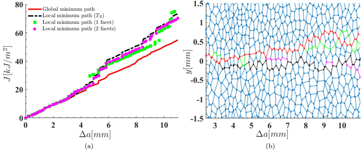
Fig. 3 The (a) crack growth resistance curves and corresponding (b) crack paths predicted using three local minimum crack growth resistance criteria and the global minimum crack growth resistance criterion.
