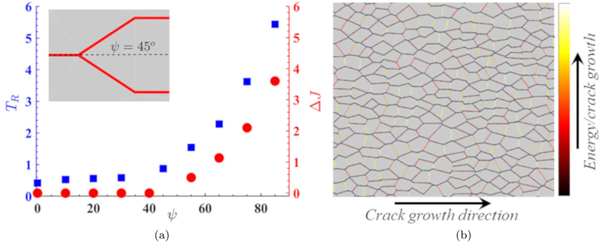
Fig. 2 (a) The tearing modulus, T_R , of a crack propagating along a grain boundary oriented at an angle \psi with respect to the plane of the propagating crack (closed squares) and the increment in crack growth initiation resistance, \Delta J , resulting from a crack reaching a triple junction as a function of \psi (closed circles). The inset in (a) shows a symmetric triple junction placed directly in front of the initial crack with an opening angle \psi = 45^\circ . (b) A schematic representation of the graph describing the change in J required for the crack to propagate through the grain boundary network. The edges of the graph representing grain boundary \alpha network are colored by the value of the required \Delta J to propagate through the grain boundary facet.
