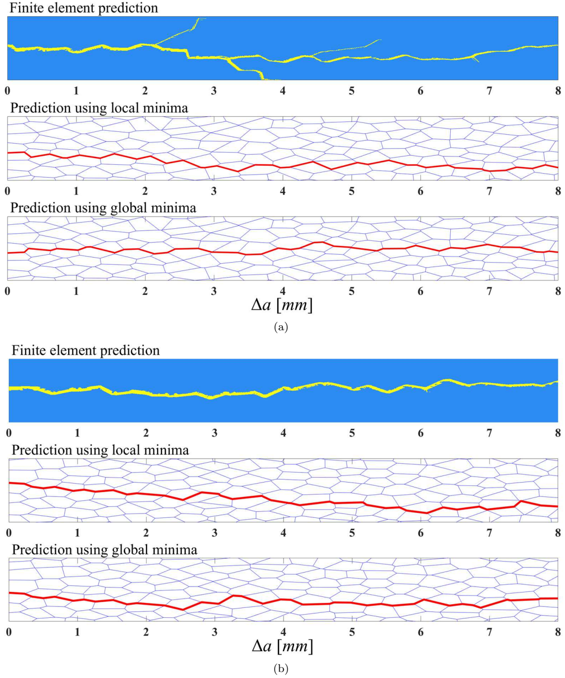
Fig. 5 Crack paths obtained from the microstructure-based finite element calculations and predicted using the proposed model based on global minimum crack growth resistance and local minimum crack growth resistance for two realizations of the specified grain microstructure: (a) realization 1 and (b) realization 2.
