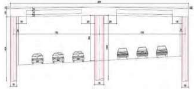
Fig. 2. Drilling section
