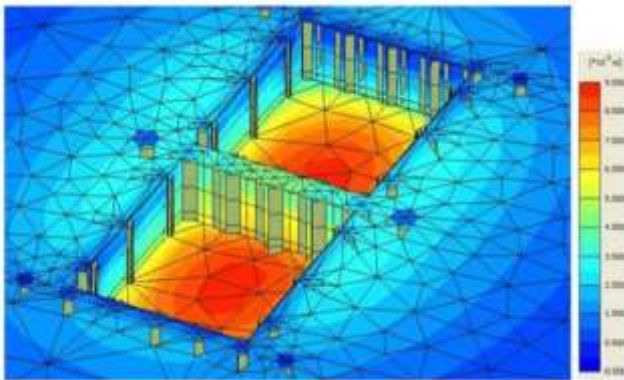
Fig. 12. settlement after 3.5 meters of drilling
