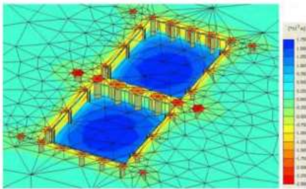
Fig. 11. settlement after 2 meters of drilling
