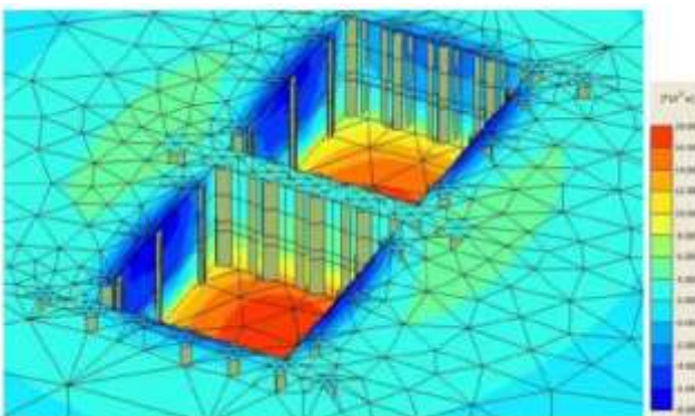
Fig. 13. settlement after 5.5 meters of drilling
