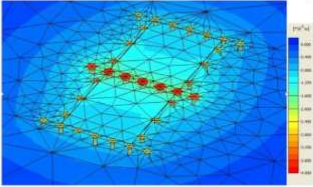
Fig. 10. Shift the ground level after placing the piles
