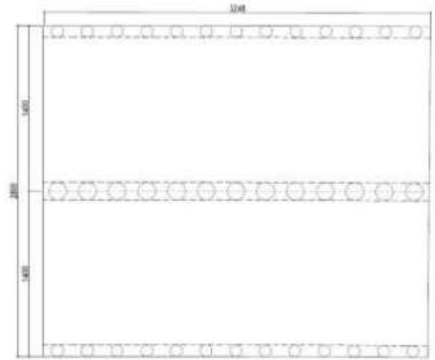
Fig. 3. The position of the piles
