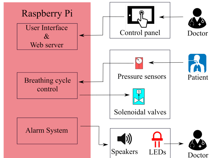
Figure 5: Control diagram for the interactions between doctors, patients and the ventilator. Raspberry Pi is used for both the user interface and communications with the electronics.
