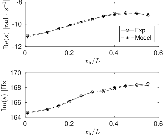
FIGURE 7: Decay rate (top) and frequency (bottom) of acoustic oscillations when the heater is switched off and placed at different x_h/L . The calibrated heater parameters are: k_{vis,h} = 27.3 \text{ kg m}^{-2} \text{ s}^{-1} , k_{th,h} = 1.53 \cdot 10^{-5} \text{ kg}^{-1} \text{ m}^2 \text{ s} , \tau_{vis,h} = -1.36 \cdot 10^{-3} \text{ s} , and \tau_{th,h} = 8.98 \cdot 10^{-4} \text{ s} .
