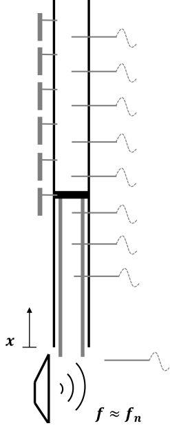
FIGURE 1: Sketch of the experimental apparatus including 6 microphones, 8 thermocouples to measure the gas temperature at the tube centerline, a thermocouple to measure the ambient temperature, a loudspeaker, and an electric heater held in place by a pair of prongs and wires. Note that the loudspeaker acoustically forces the system at a frequency, f , close to the natural frequency of the tube, f_n .
