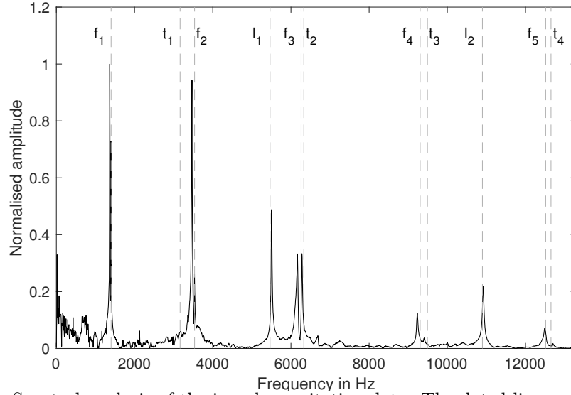
Figure 6: Spectral analysis of the impulse excitation data. The dotted lines mark natural frequencies based on FEM calculations. The Young's and shear modulus of the FEM material model result from a error minimisation between the peaks in the spectrum and the calculated eigenfrequencies ( <12 kHz)
