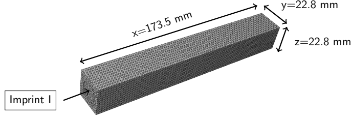
Figure 3: Meshed specimen for FEM calculation of natural frequencies and eigenmodes.
