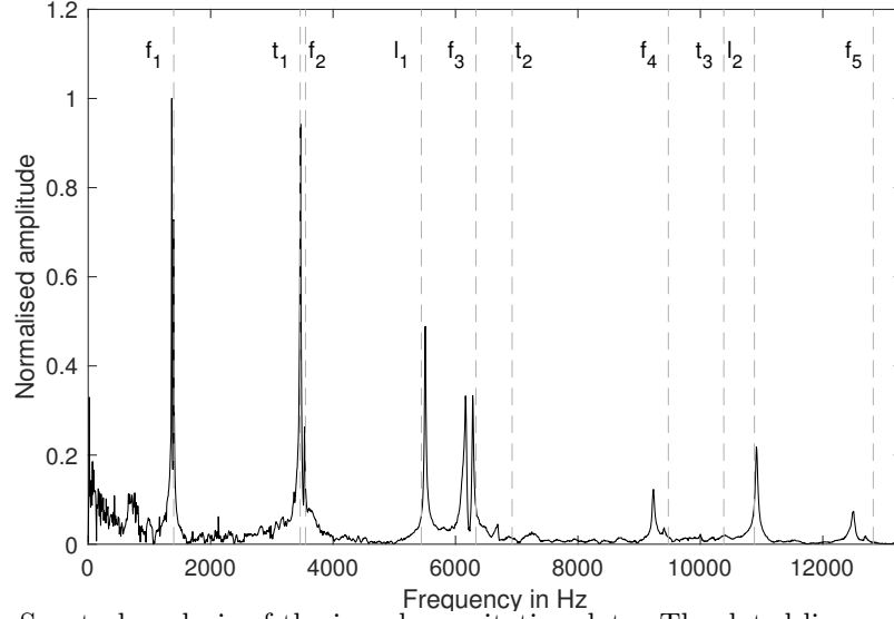
Figure 5: Spectral analysis of the impulse excitation data. The dotted lines mark natural frequencies based on FEM calculations, with Young's modulus and the shear modulus calculated analytically using f_1 and t_1 , respectively.
