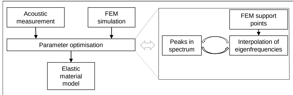
Figure 2: Algorithm for determining elastic parameters via impulse excitation technique and FEM simulation. The measured and calculated eigenfrequencies are compared and the Young's modulus and Poisson number are optimised such, that the error between the measured and the calculated eigenfrequencies is minimal.
