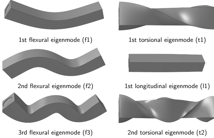
Figure 4: Eigenmodes 1-6 of the specimen obtained by FEM simulation
