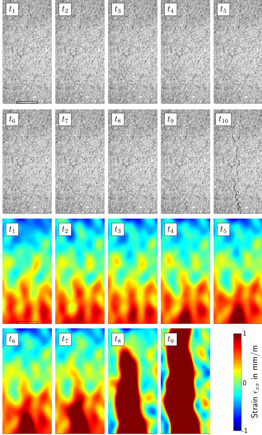
Figure 7: Strain calculation via digital image correlation for a 3PB experiment and 10 points in time ( t_1 - t_{10} ). Only the area under the punch is analysed. Starting at t_2 , the strain starts to localise until the fracture is complete at t_9 , which is still undetectable by the human eye.
