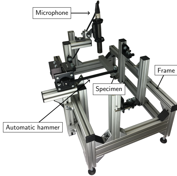
Figure 1: Test-bench for determining elastic properties via impulse excitation technique. The main components are a microphone, a specimen, an automatic hammer system and the frame of the test-bench.
