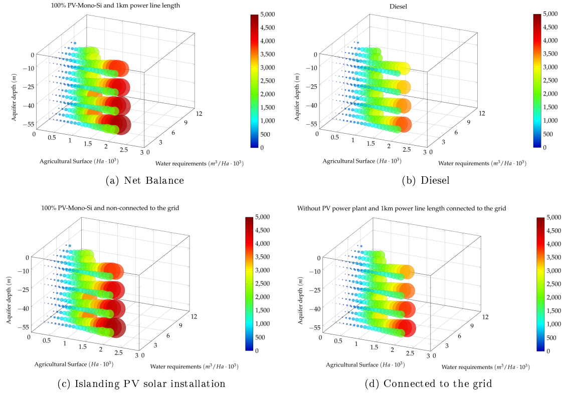
Figure 9: Estimated Required Direct Pumping Power (kW). Comparison of solutions
