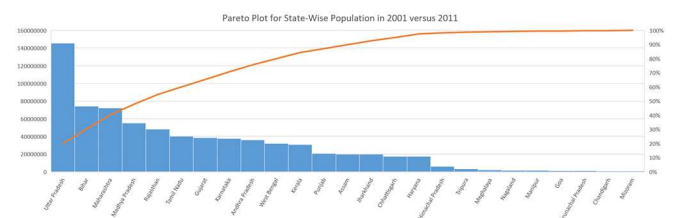
Fig. 13. Pareto Plot showing State versus population for the years 2001 and 2011.
